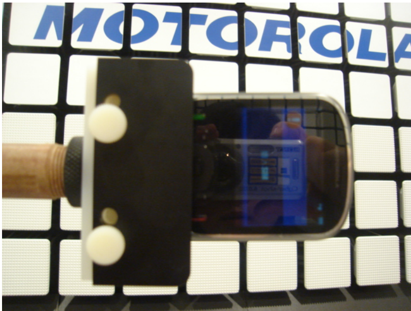
22708-1, IHDT56KE1 placed in test position Y – slider closed
