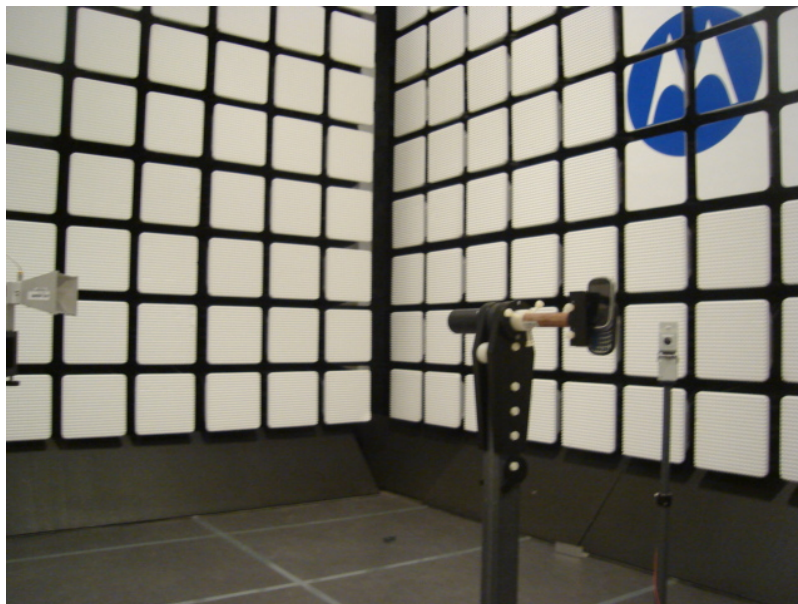
22708-1, IHDT56KE1 setup in semi-anechoic chamber – right view (18 GHz – 26.5 GHz)
