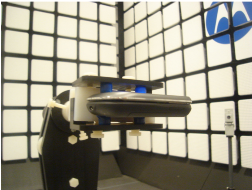
22708-1, IHDT56KE1 placed in test position X – slider closed
