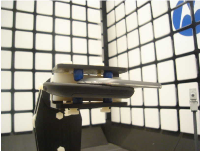
22708-1, IHDT56KE1 placed in test position X – slider open
