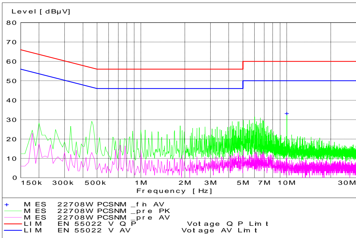
WCDMA PCS Channel 9400 - Tx Mode - Neutral Coupling
