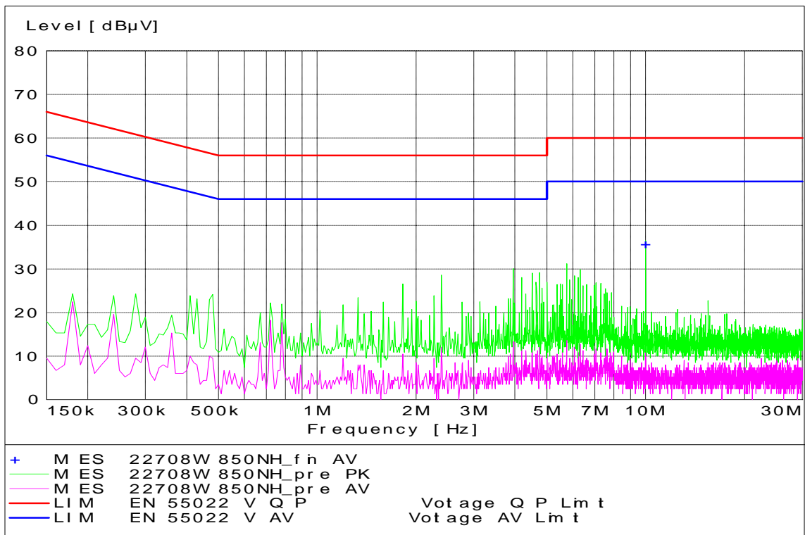
WCDMA 850 Channel 4233 - Tx Mode - Neutral Coupling
