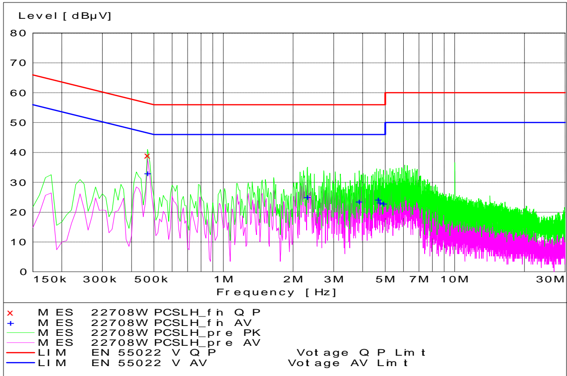
WCDMA PCS Channel 9538 - Tx Mode - Line Coupling
