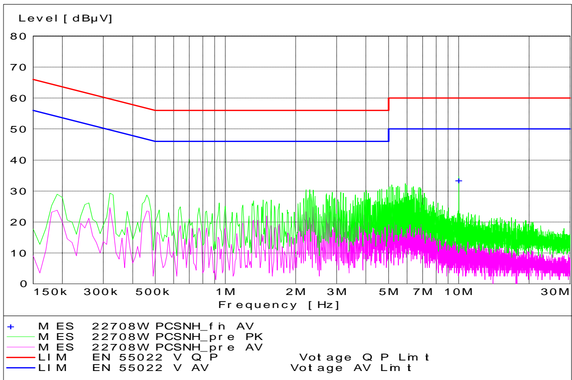
WCDMA PCS Channel 9538 - Tx Mode - Neutral Coupling
