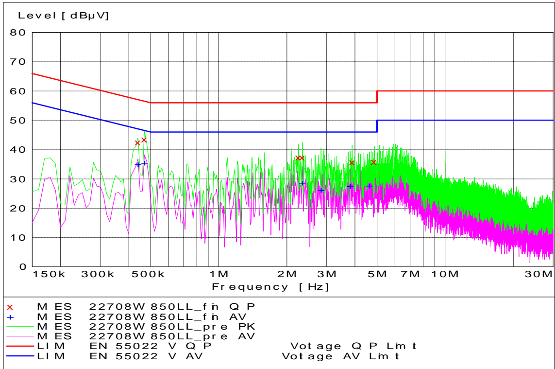
WCDMA 850 Channel 4132 - Tx Mode - Line Coupling
