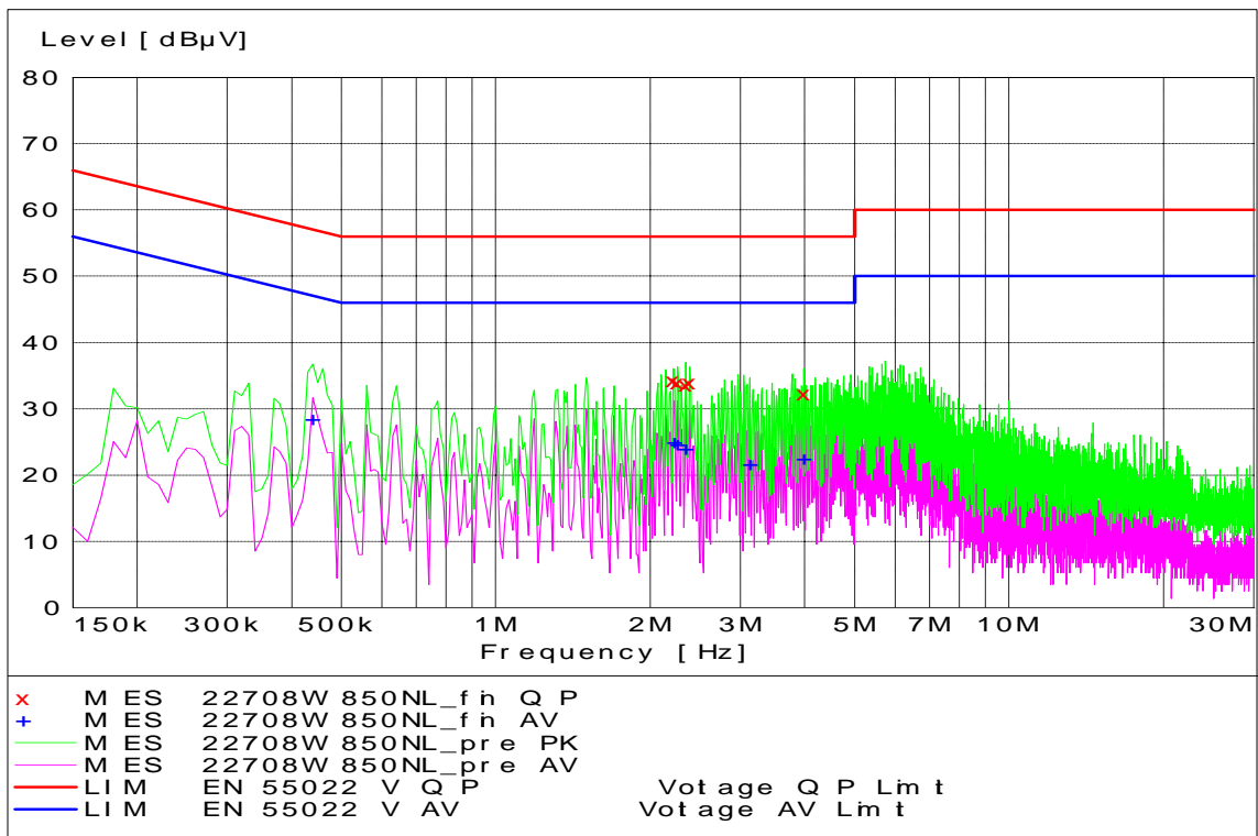
WCDMA 850 Channel 4132 - Tx Mode - Neutral Coupling
