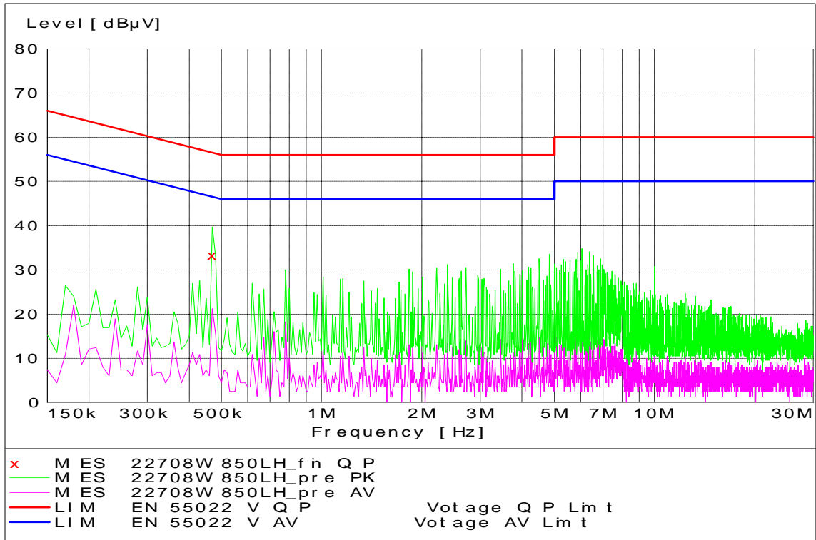
WCDMA 850 Channel 4233 - Tx Mode - Line Coupling
