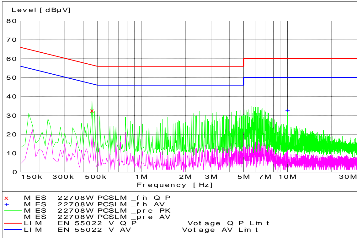
WCDMA PCS Channel 9400 - Tx Mode - Line Coupling
