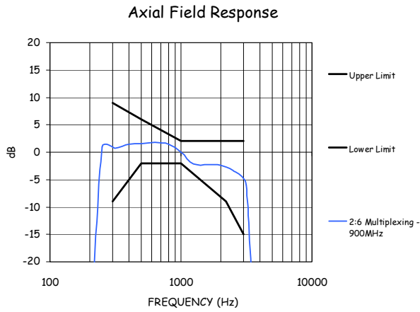
Figure 9-1-3: 900 MHz Measured Frequency Response (2:6).
