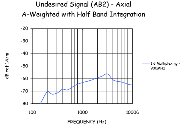
Figure 9-4-2: 900 MHz Undesired Signal (1:6).
