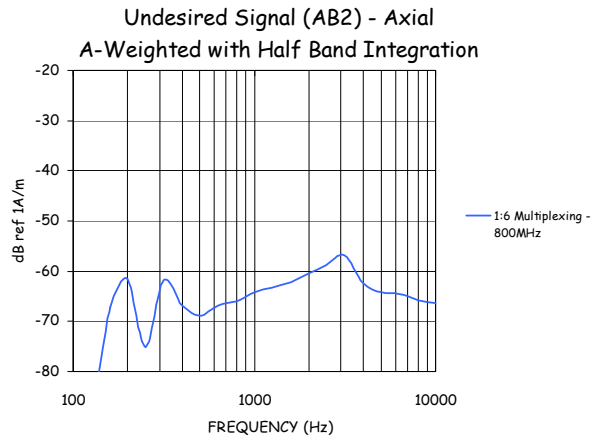
Figure 9-2-2: 800 MHz Undesired Signal (1:6).
