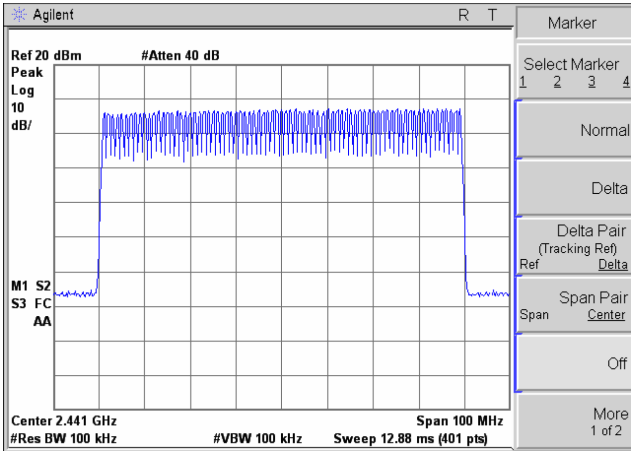
Figure 6c.3-1: Plot of number of Bluetooth hopping frequencies
