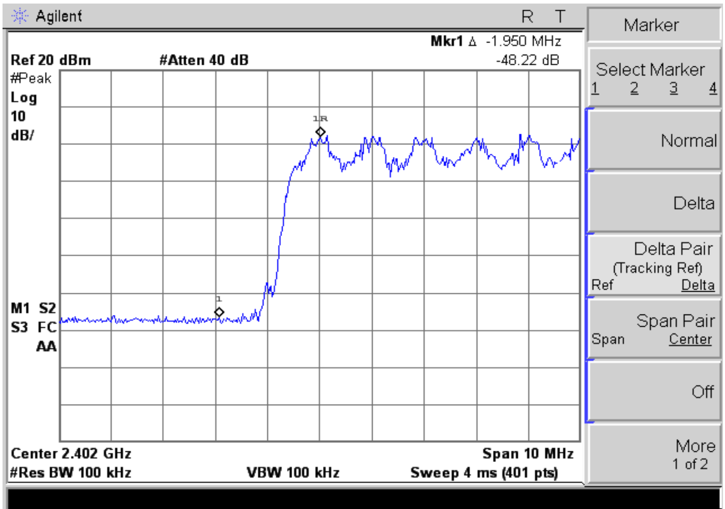
Figure 6c.6-11: Plot of lower band-edge conducted emissions with hopping enabled (8 DPSK Modulation).
