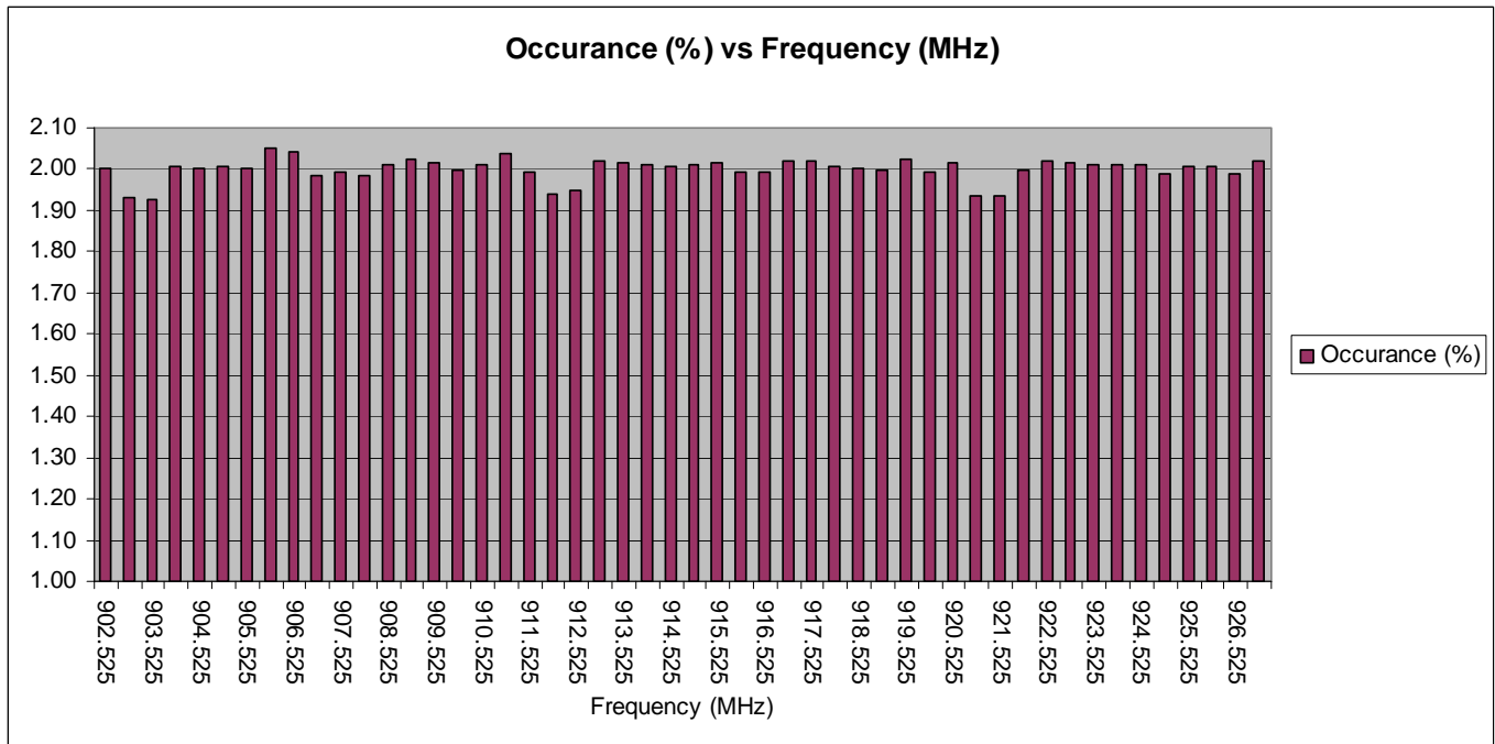
Figure 6b.2.7.1. Histogram of MOTotalk ISM Band Discontinuous Transmissions.
