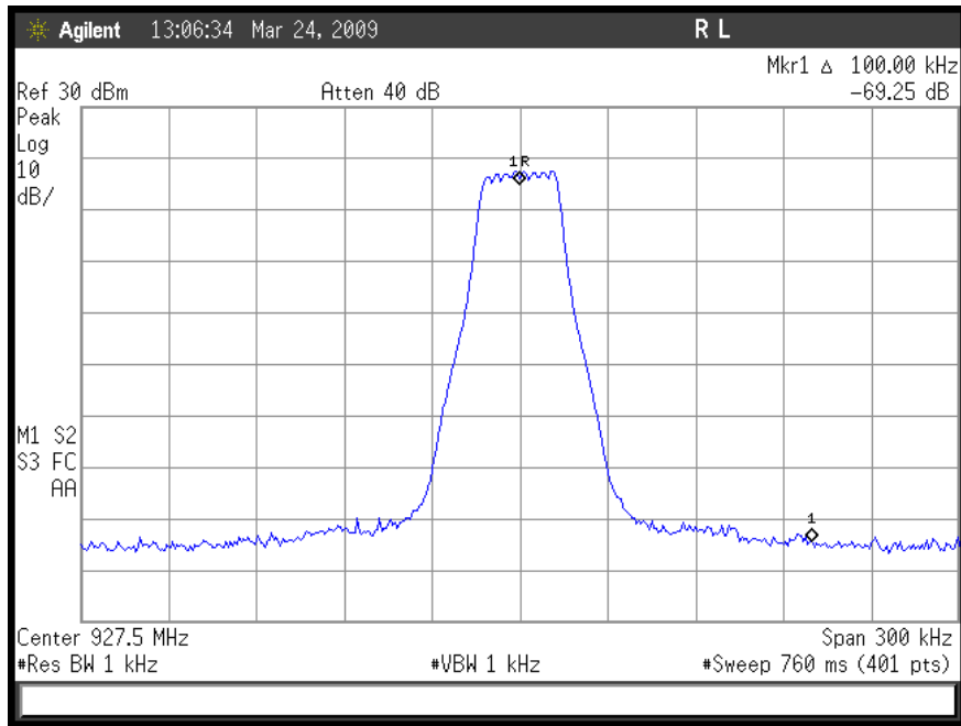
Figure 6b.2.2.7 MOTotalk ISM band occupied bandwidth with frequency span of 300 kHz with hopping function disabled, at center frequency 927.475.
