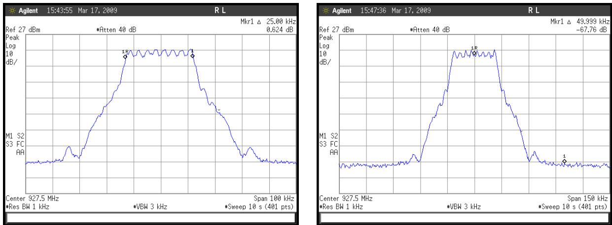
Figure 6b.2.2.5 Spectrum analyzer plot of MOTotalk ISM Band 8-FSK traffic channel signal’s 99% bandwidth with hopping function disabled, at center frequency 927.475 MHz.
