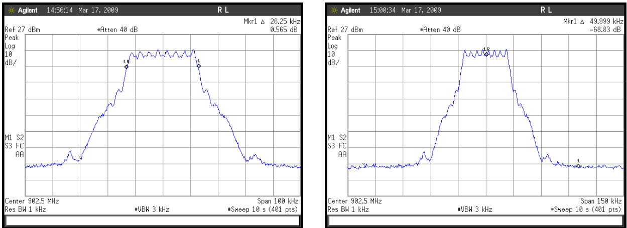
Figure 6b.2.2.1 Spectrum analyzer plot of MOTotalk ISM Band 8-FSK traffic channel signal’s 99% bandwidth at center frequency 902.525 MHz, with hopping function disabled.
