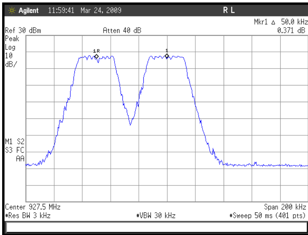
Figure 6b.2.2.6. Adjacent hop set separation with spectrum analyzer center frequency 927.5 MHz.
