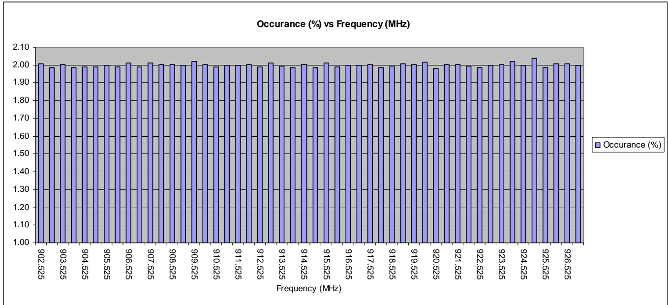
Figure 6b.2.6.1. Histogram of MOTotalk ISM Band Continuous Transmission.
