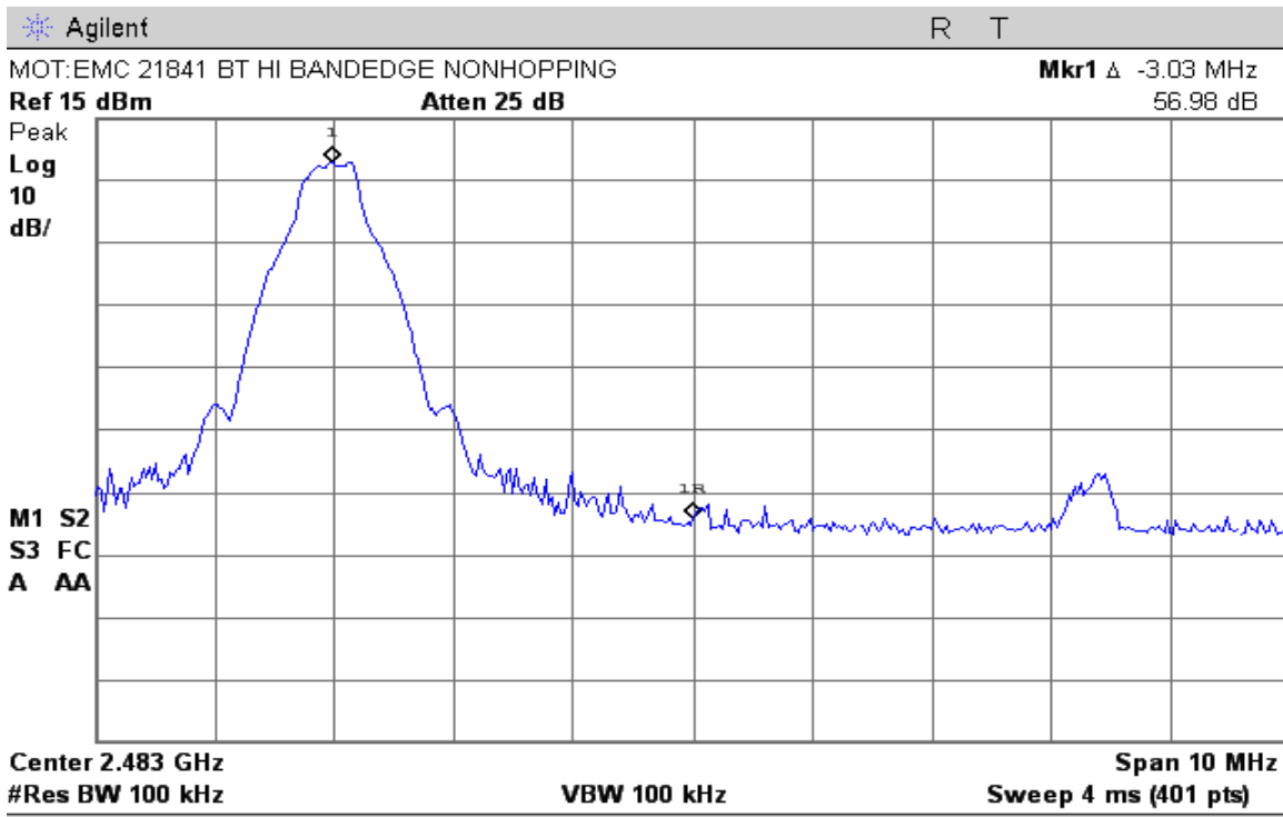
High Band Edge with Hopping disabled and EDR Mode disabled
