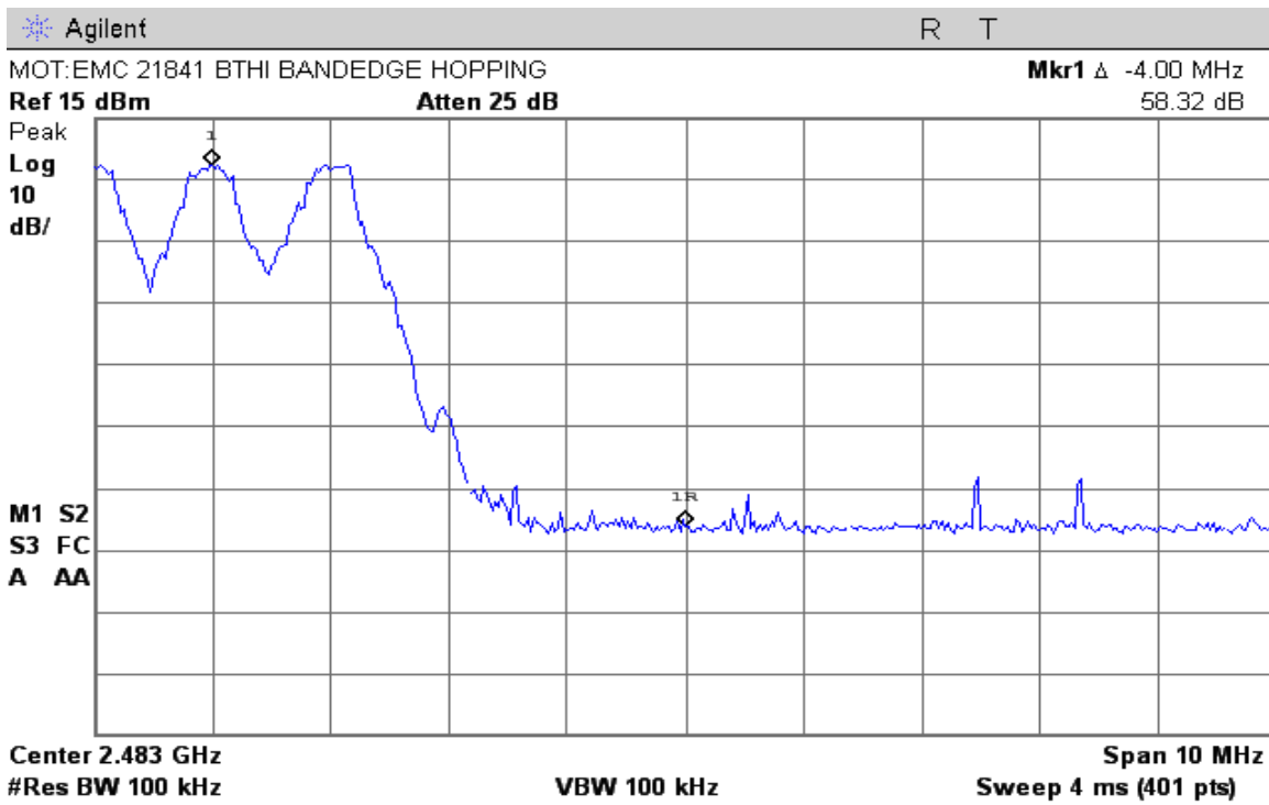
High Band Edge with Hopping enabled and EDR Mode disabled
