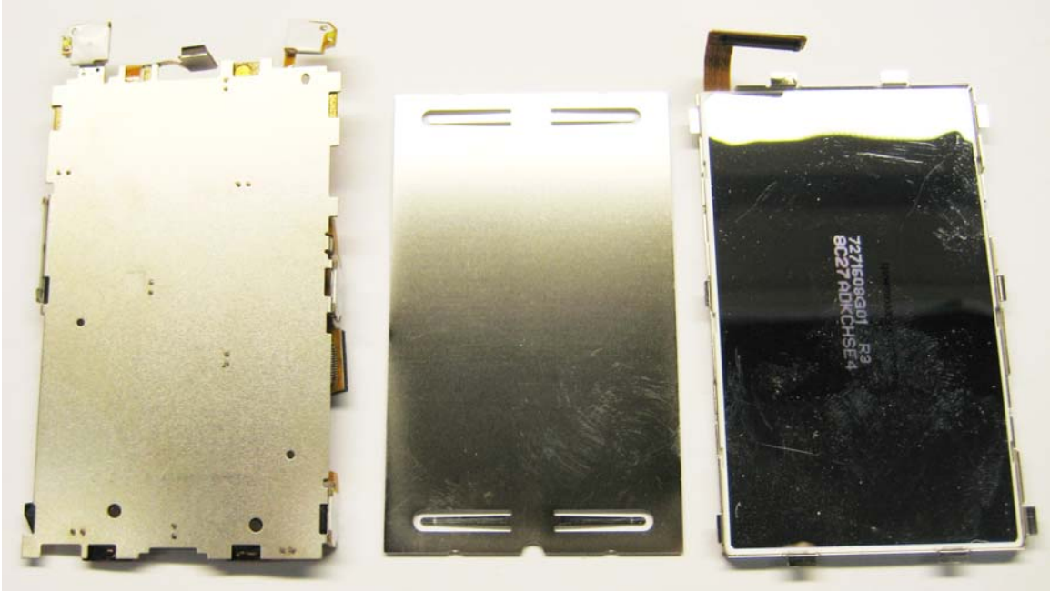
Display assembly
