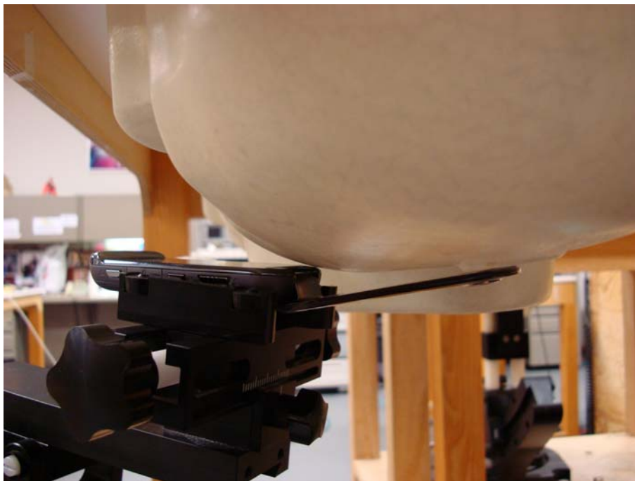
Figure 4 – Transceiver against head, Cheek Touch position
