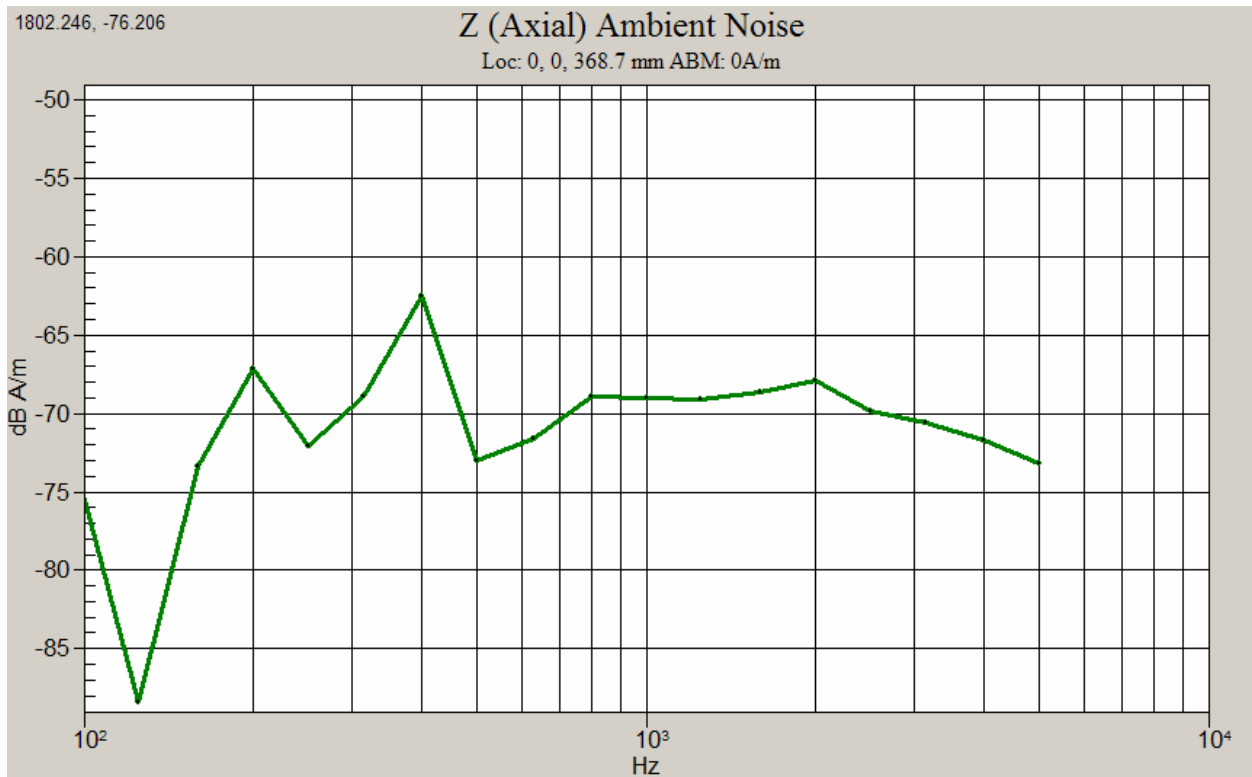
Graph A2-1. Axial Position Ambient Noise Spectrum Plot
