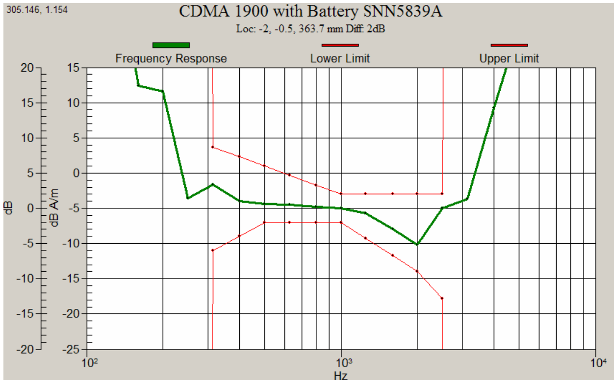
Graph 4: CDMA 1900 Frequency Response with Battery 2
