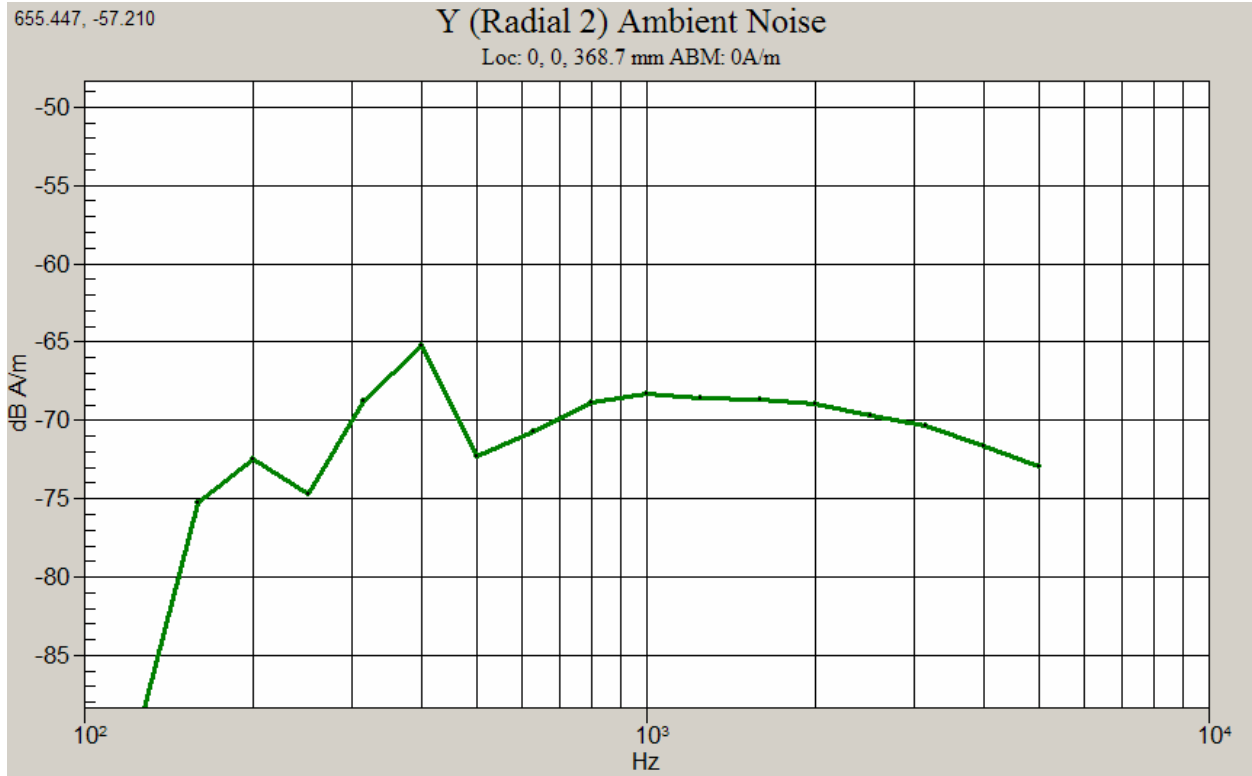
Graph A2-3. Radial 2 Position Ambient Noise Spectrum Plot
