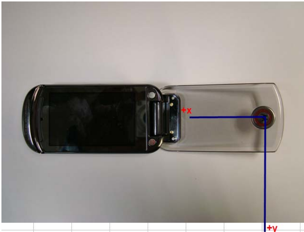
Figure 6. Coordinate Axis for T-coil Measurements
