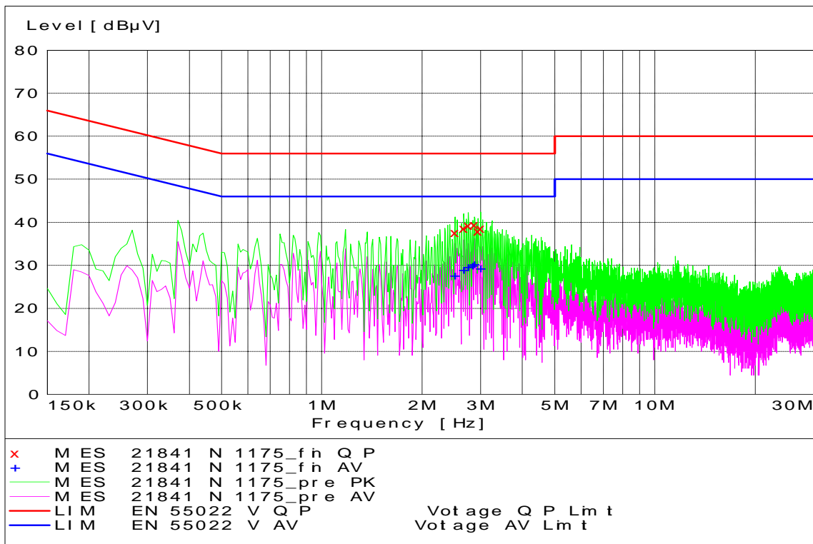
EVDO PCS Channel 1175 - Tx Mode - Neutral Coupling
