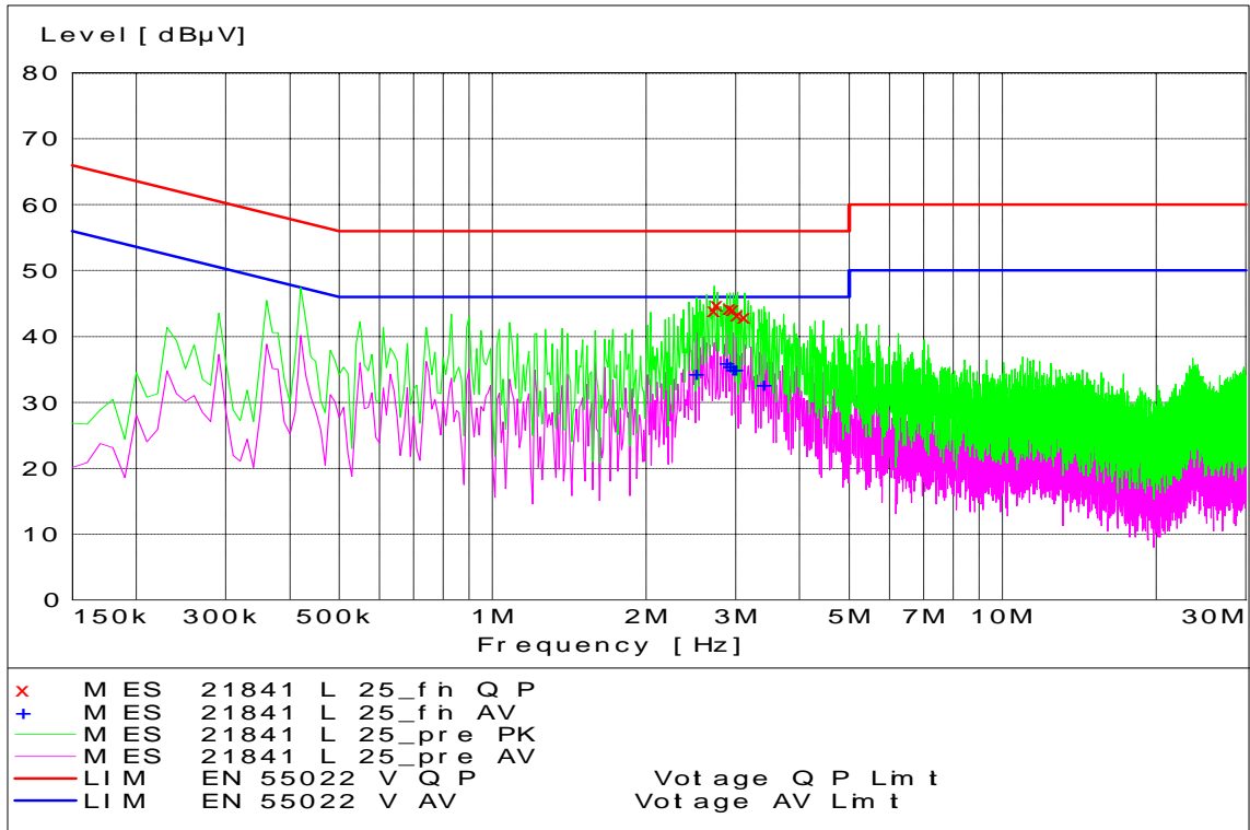
EVDO PCS Channel 25 - Tx Mode - Line Coupling
