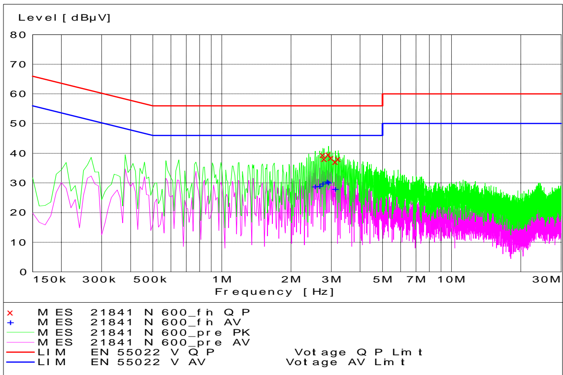
EVDO PCS Channel 600 - Tx Mode - Neutral Coupling
