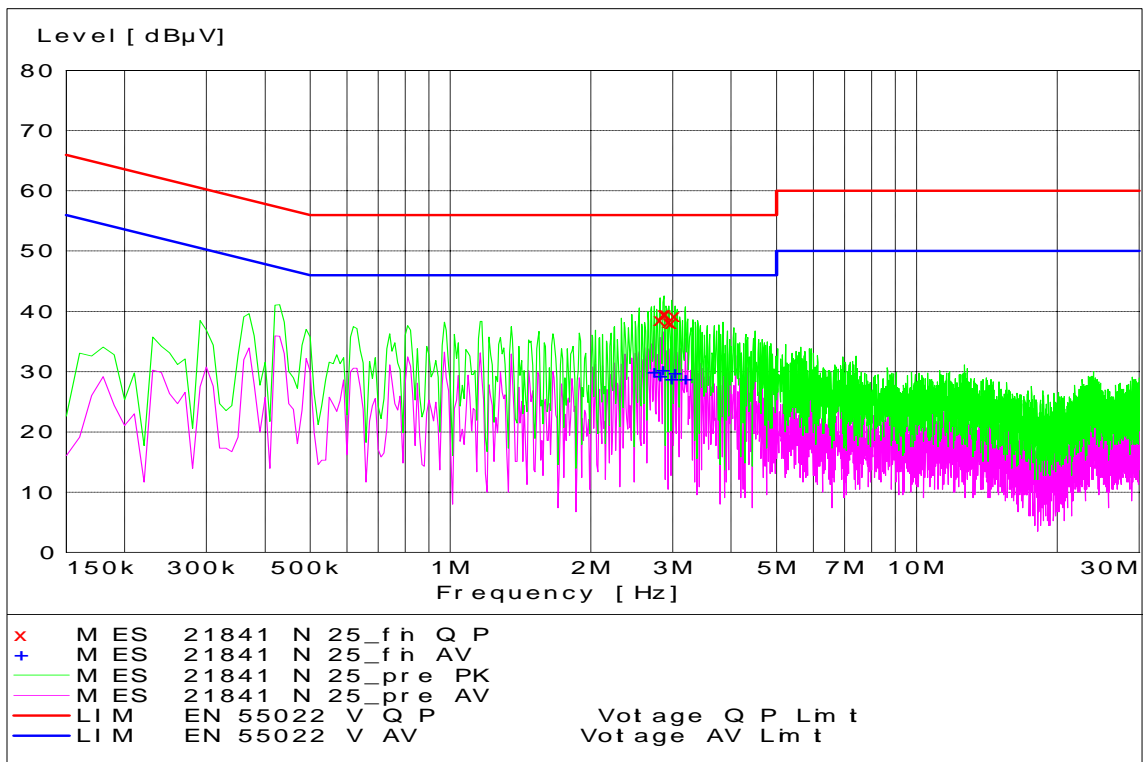
EVDO PCS Channel 25 - Tx Mode - Neutral Coupling
