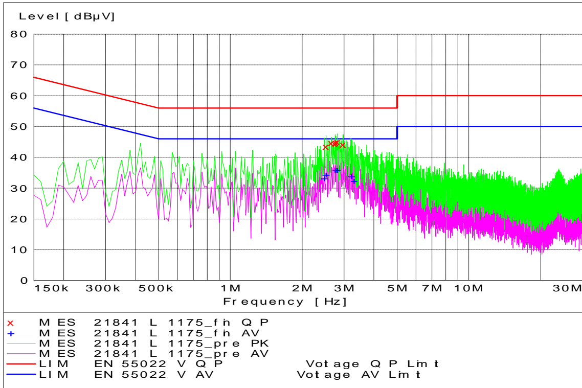
EVDO PCS Channel 1175 - Tx Mode - Line Coupling
