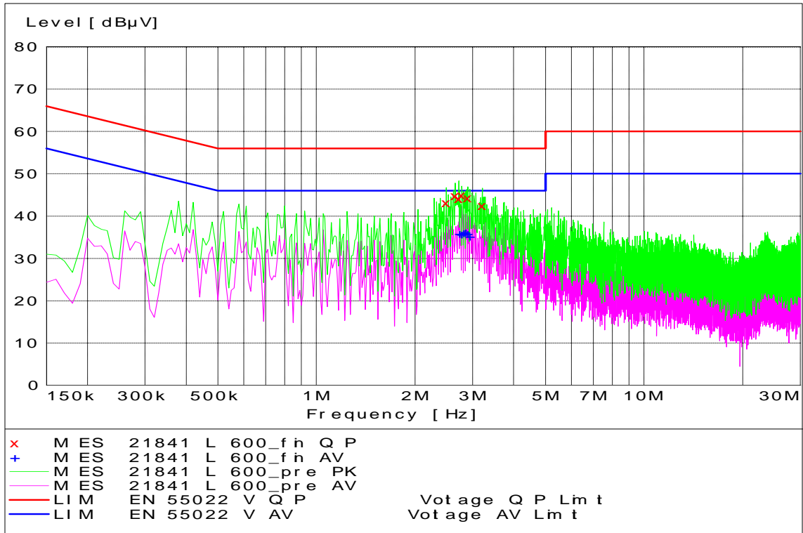
EVDO PCS Channel 600 - Tx Mode - Line Coupling
