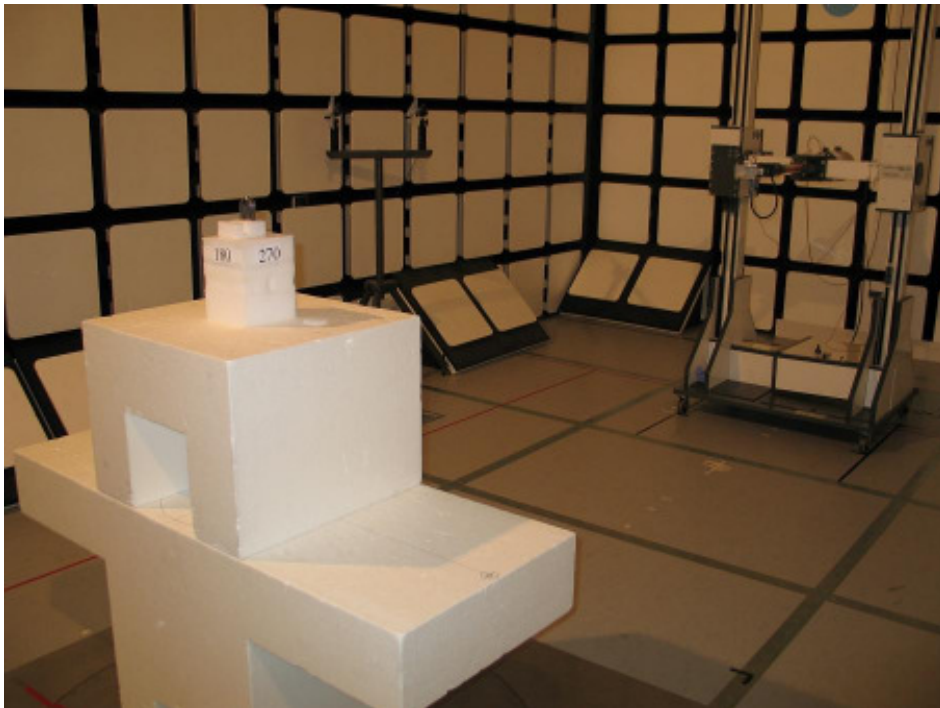
22268-1, IHDT56JY1 setup in semi-anechoic chamber – right side
