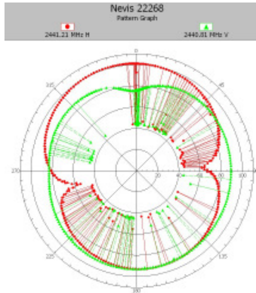
22268-1, IHDT56JY1 maximum radiation pattern position Z - closed
