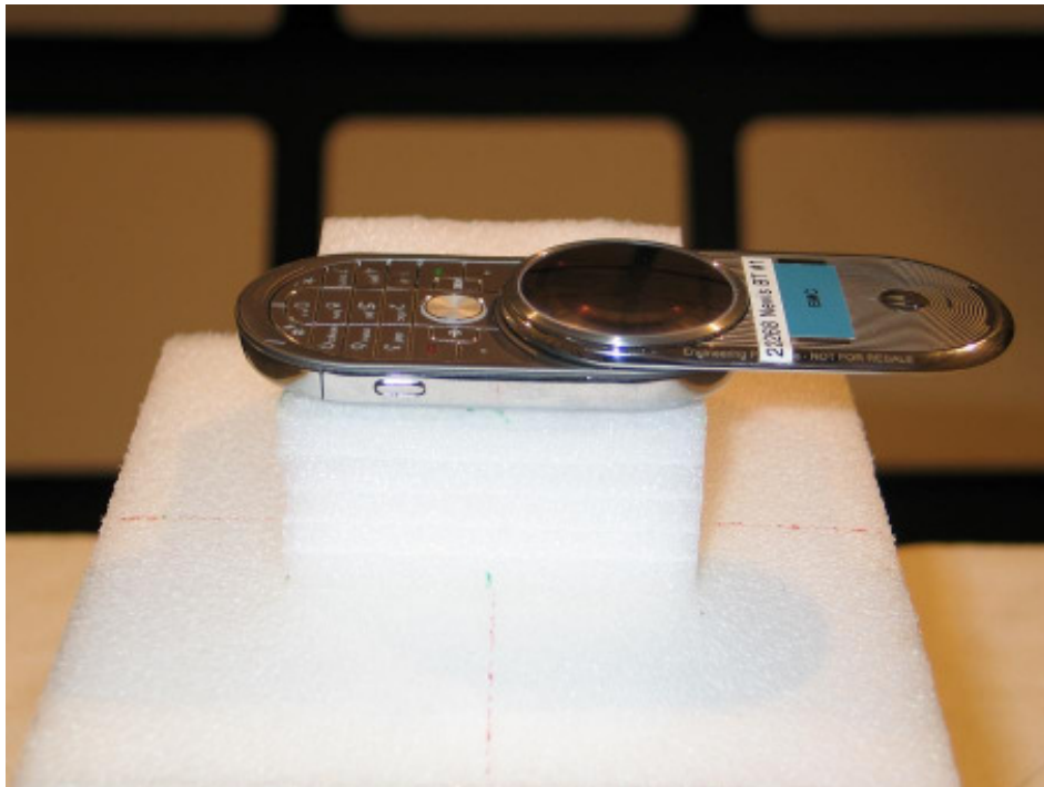
22268-1, IHDT56JY1 placed in test position X - Open
