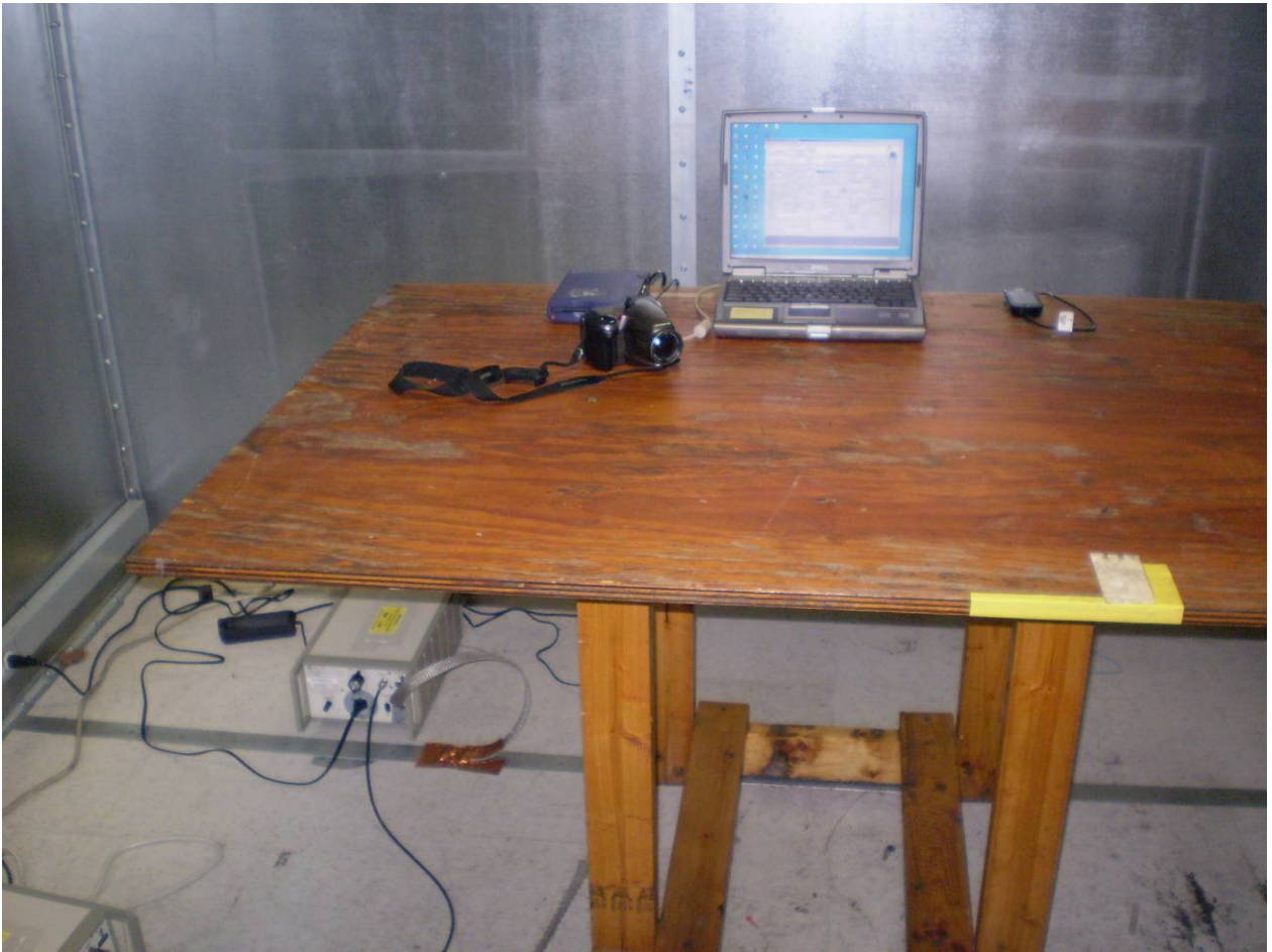
AC Line Conducted Emissions
