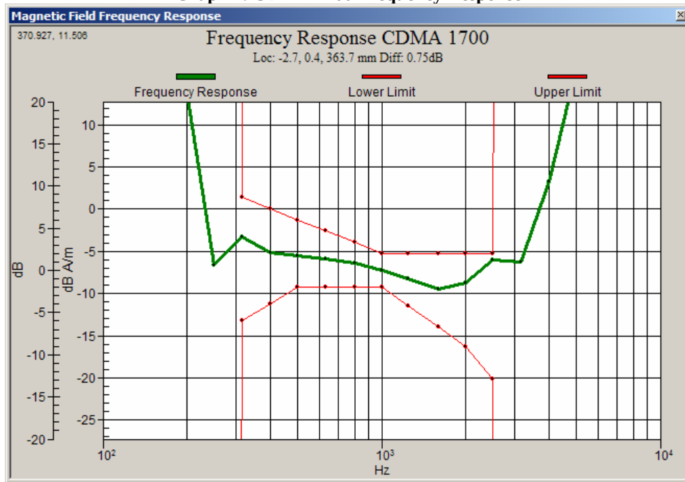
Graph 4: CDMA 1700 Frequency Response
