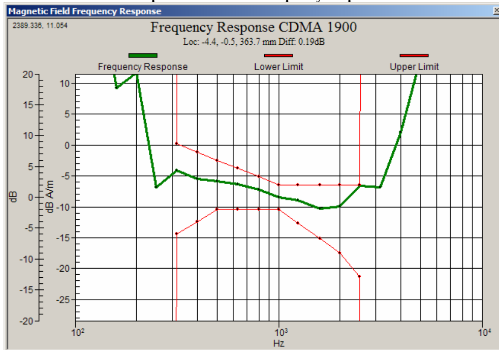
Graph 3: CDMA 1900 Frequency Response
