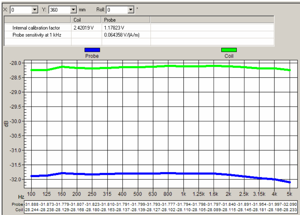
Graph 1: Frequency Response measured in AMCC
