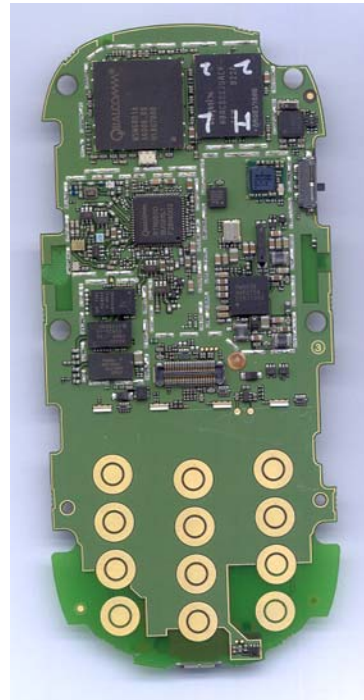
Main Board Top Without Popples
