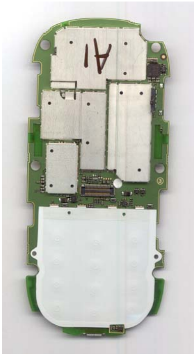
Main Board Top With Popples
