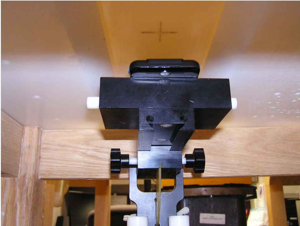
Figure 9 - Transceiver against body, 15 mm from Phantom position
