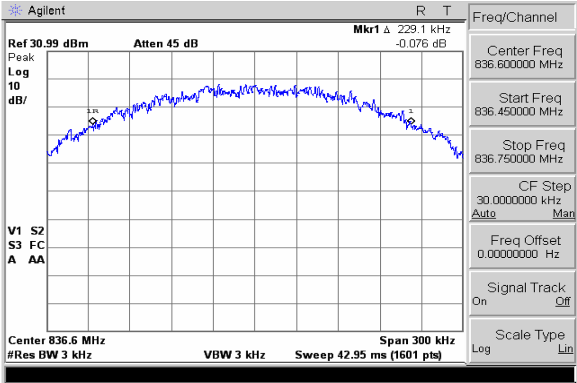
GSM 850 EDGE – Occupied Bandwidth – Channel 190 (836.6MHz)
