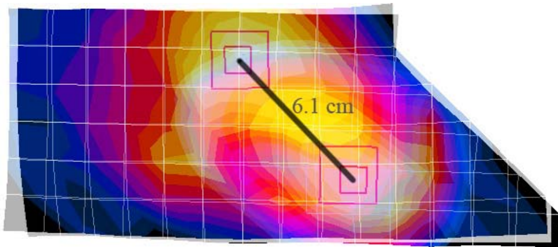
GSM850 Left Head Cheek SAR overlaid with WiFi Left Head Cheek SAR (w/ SNN5782B)
