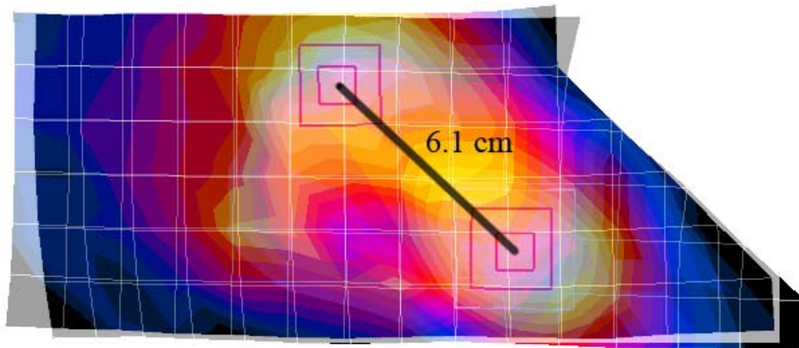
GSM1900 Left Head Cheek SAR overlaid with WiFi Left Head Cheek SAR (w/ SNN5782B)
