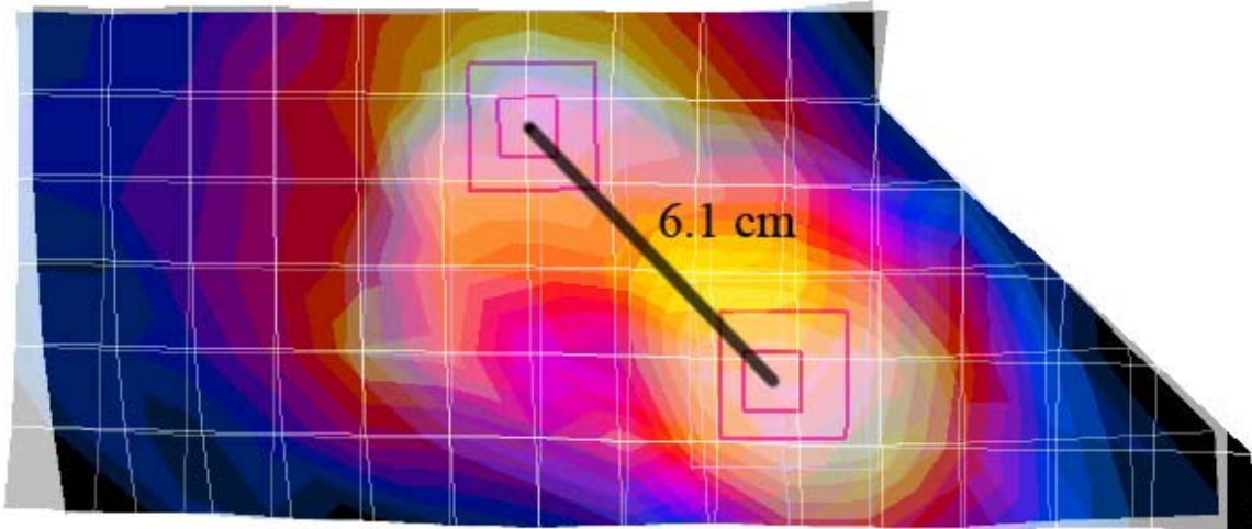
GSM1900 Left Head Cheek SAR overlaid with WiFi Left Head Cheek SAR (w/ SNN5814A)
