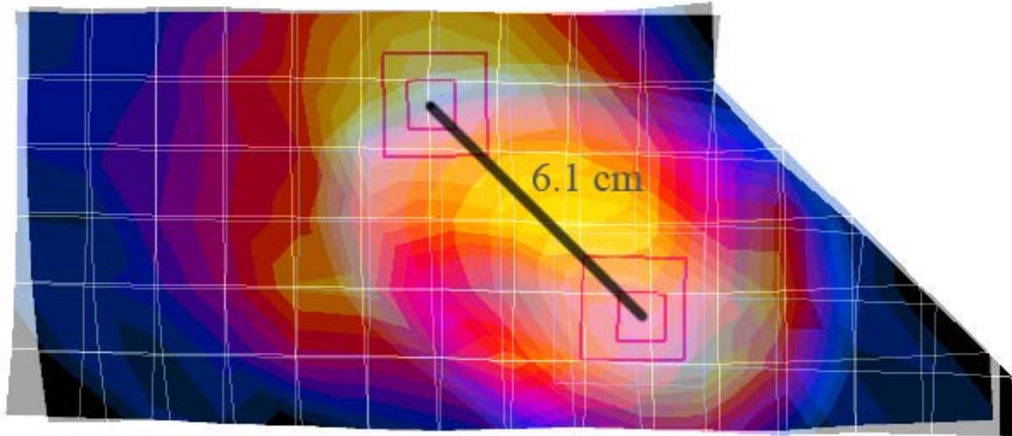
GSM850 Left Head Cheek SAR overlaid with WiFi Left Head Cheek SAR (w/ SNN5814A)
