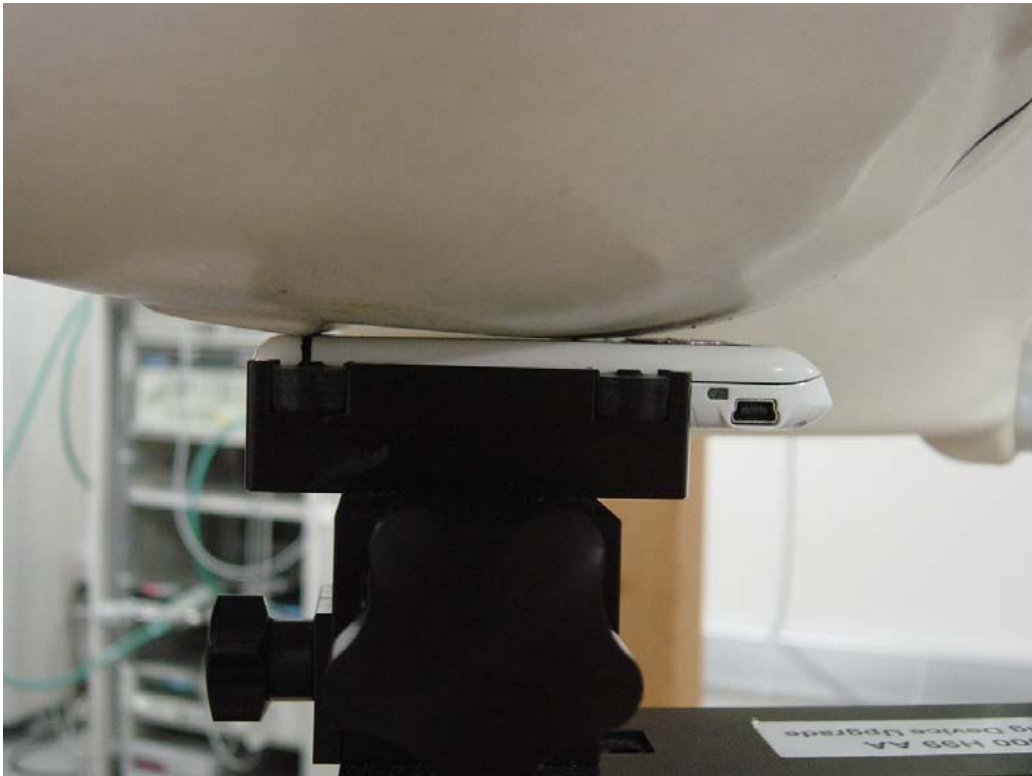
Figure 5: Phone Against Head Phantom (Cheek Touch)
