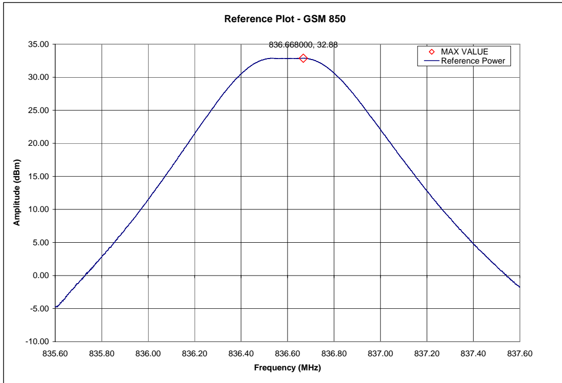
GSM 850 – Reference Level Plot – Channel 190 (836.6MHz)
