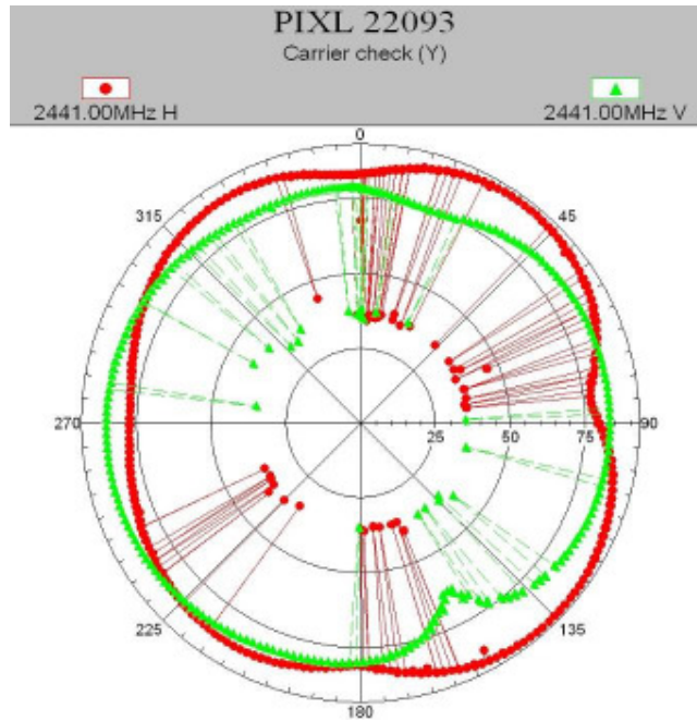
22093-1, IHDT56JT2 Maximum radiation pattern position Y
