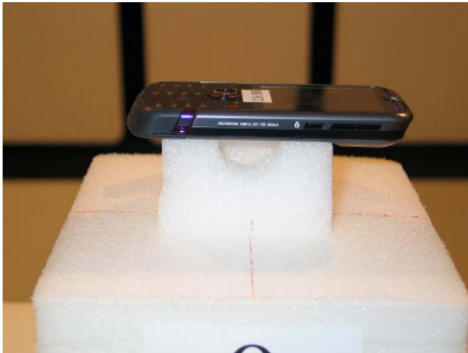
22093-1, IHDT56JT2 placed in test position X
