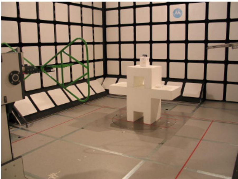
22093-1, IHDT56JT2 setup in semi-anechoic chamber – back view
