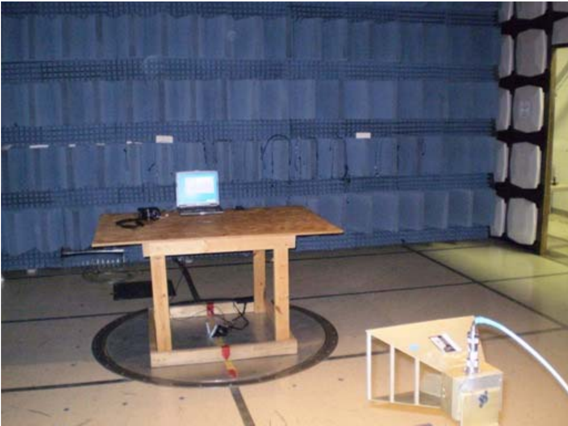
EMC Report #21653 Part 15, PC Peripheral
