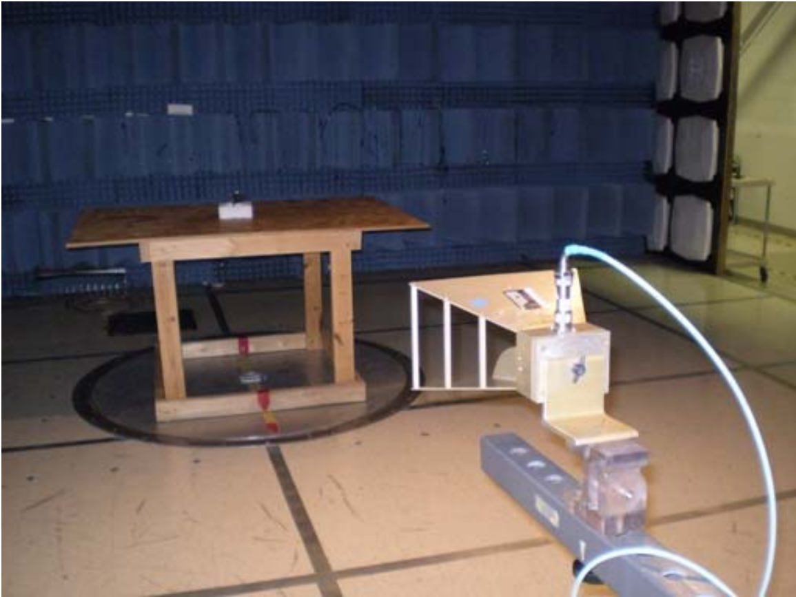
EMC Report #21653 Tx Radiated
