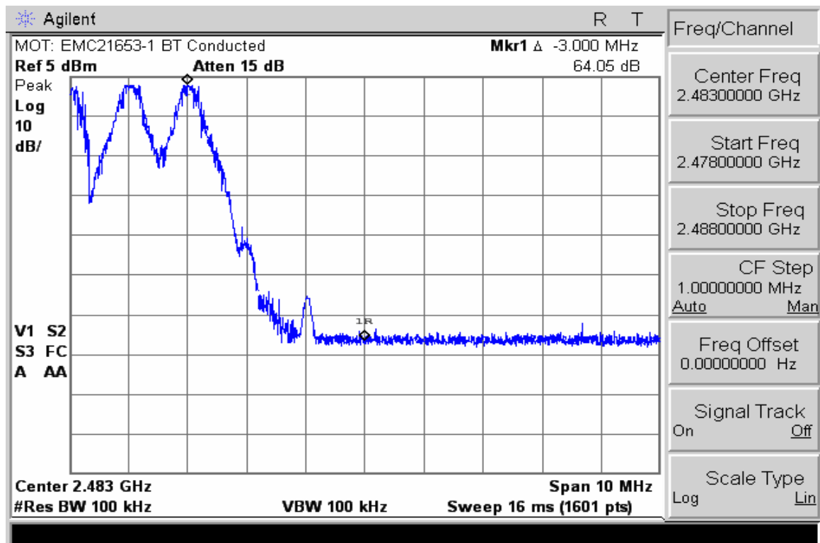
High Band Edge with Hopping enabled and EDR Mode disabled
