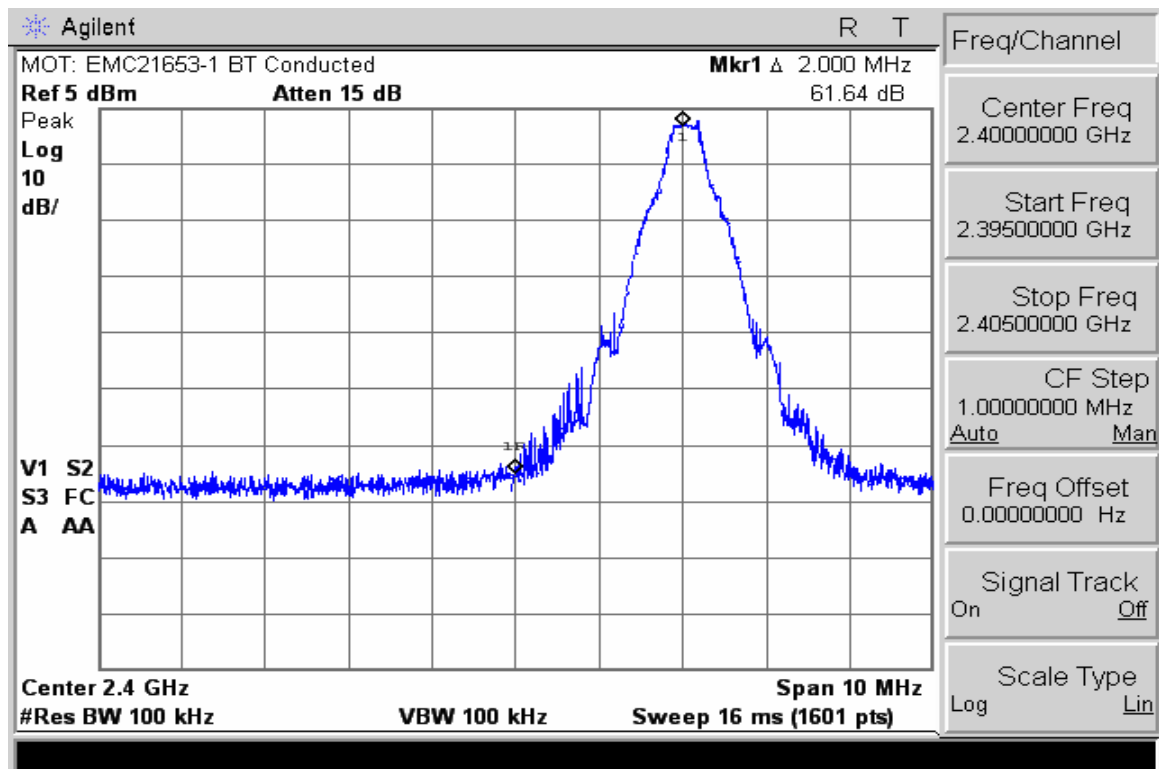
Low Band Edge with Hopping disabled and EDR Mode disabled
