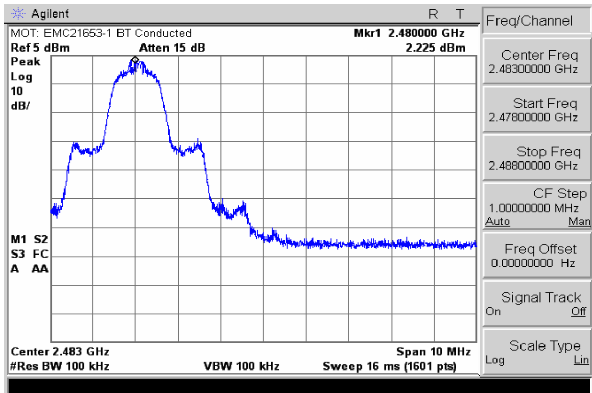
High Band Edge with Hopping disabled and EDR Mode enabled
