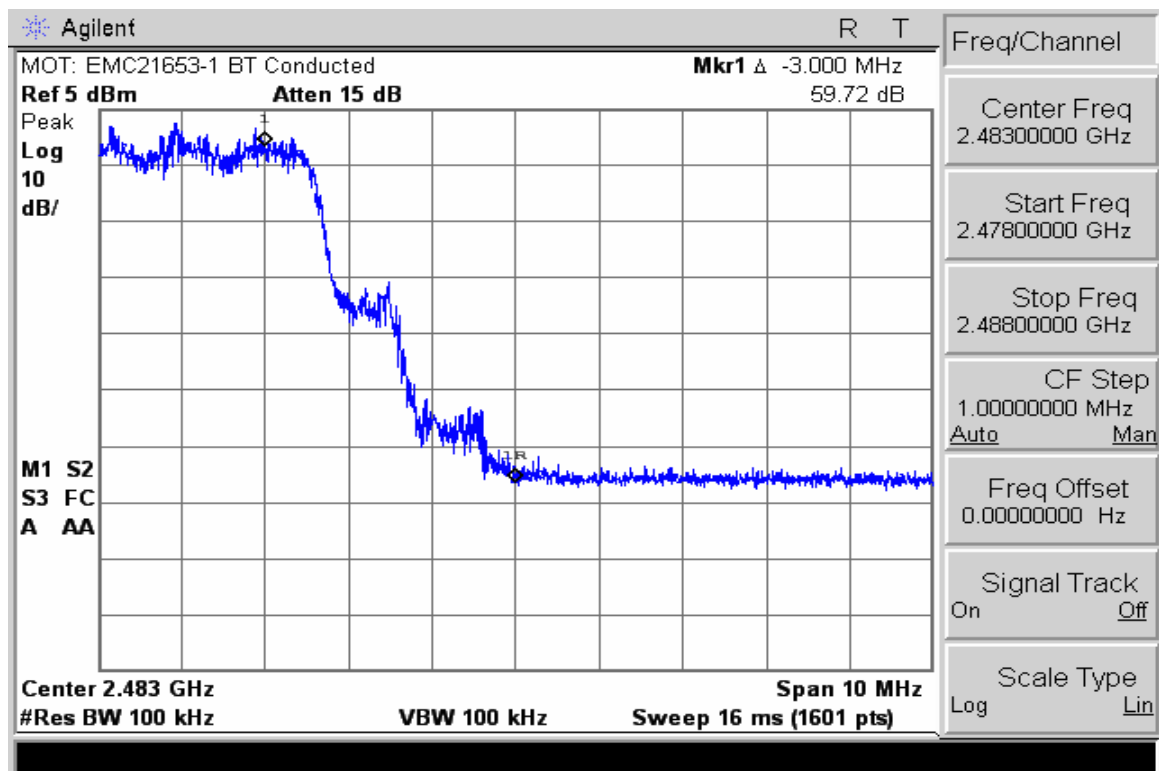
High Band Edge with Hopping enabled and EDR Mode enabled
