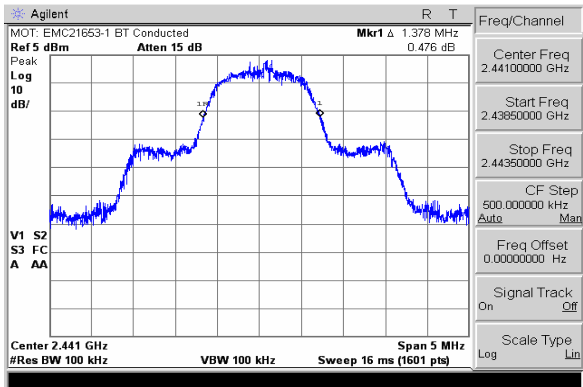
20dB Bandwidth with EDR mode enabled
