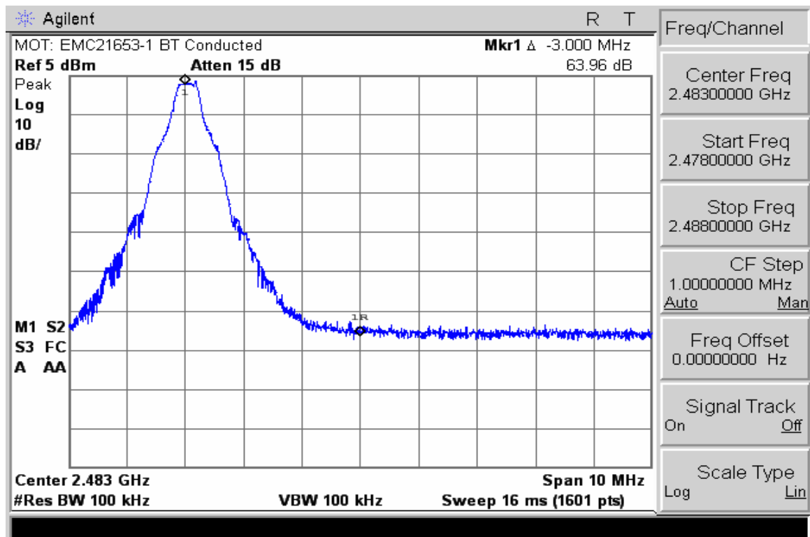
High Band Edge with Hopping disabled and EDR Mode disabled
