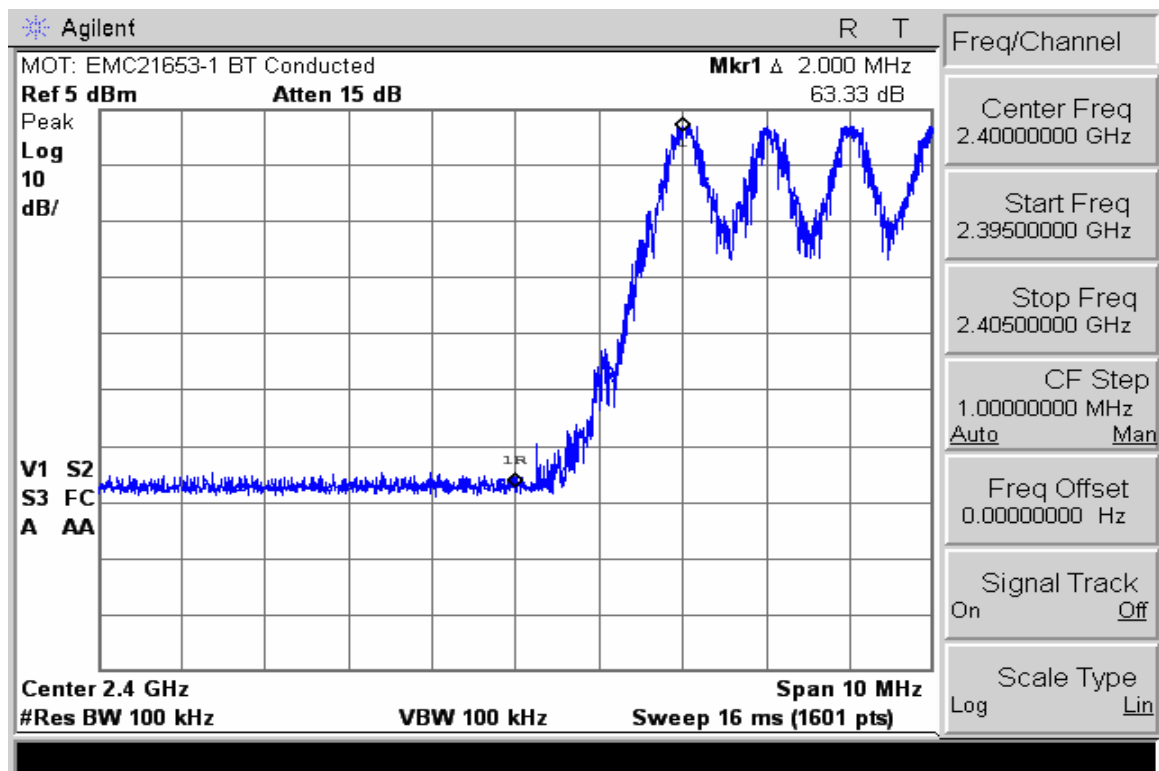
Low Band Edge with Hopping enabled and EDR Mode disabled
