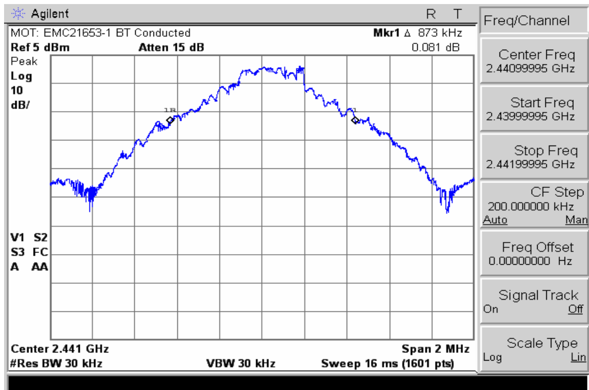
20dB Bandwidth with EDR mode disabled
