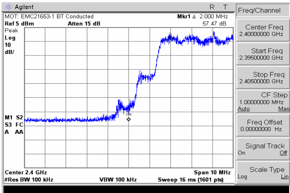
Low Band Edge with Hopping enabled and EDR Mode enabled
