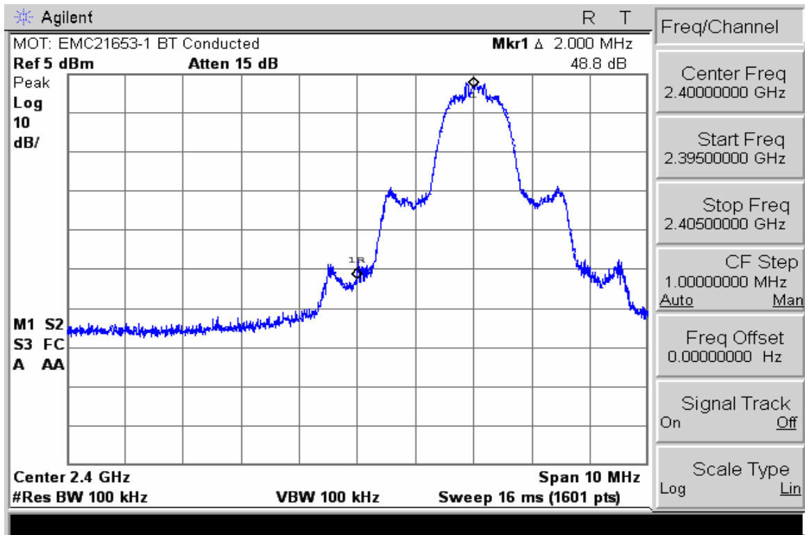
Low Band Edge with Hopping disabled and EDR Mode enabled
