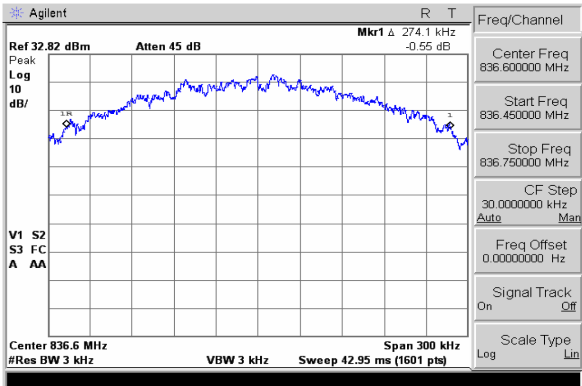
GSM 850 Occupied Bandwidth
