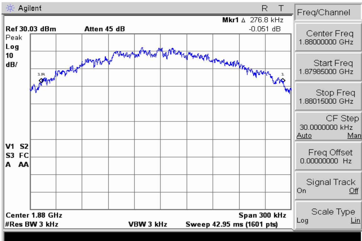
GSM 1900 Occupied Bandwidth
