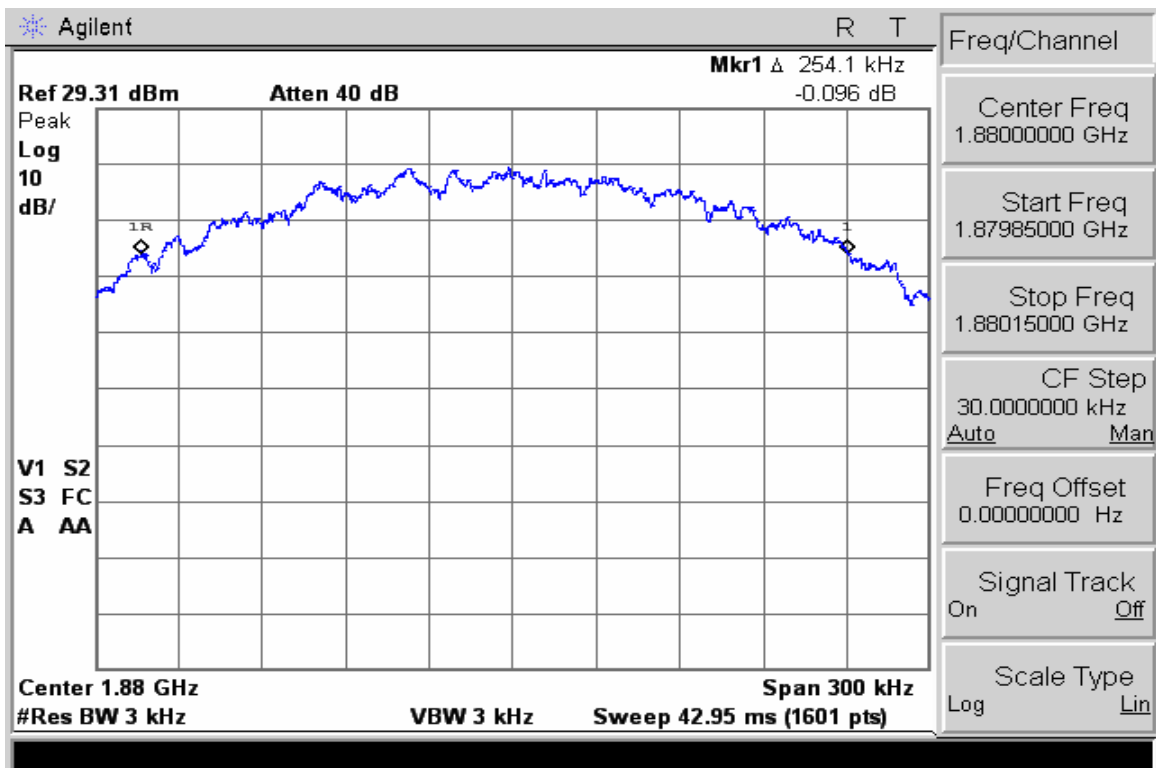
EDGE 1900 Occupied Bandwidth
