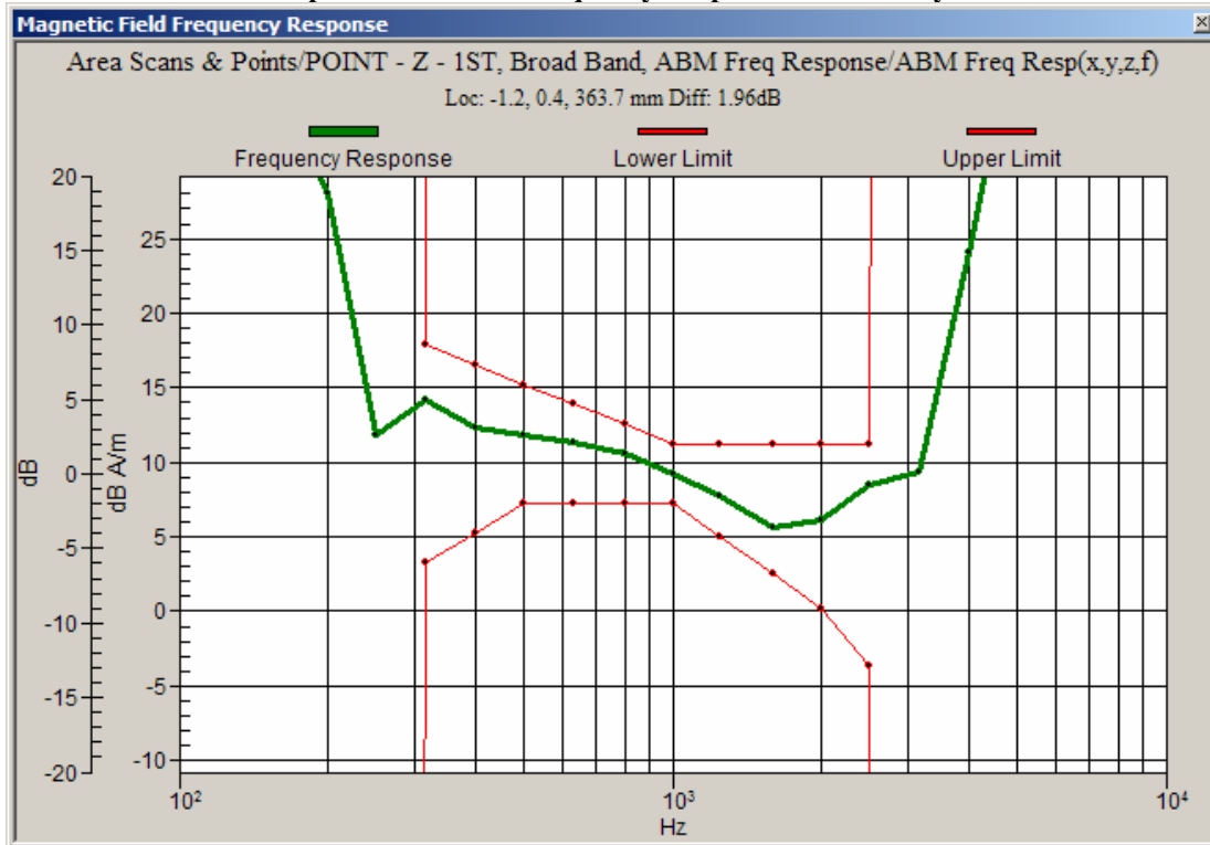
Graph 5: GSM 1900 Frequency Response with Battery 2
