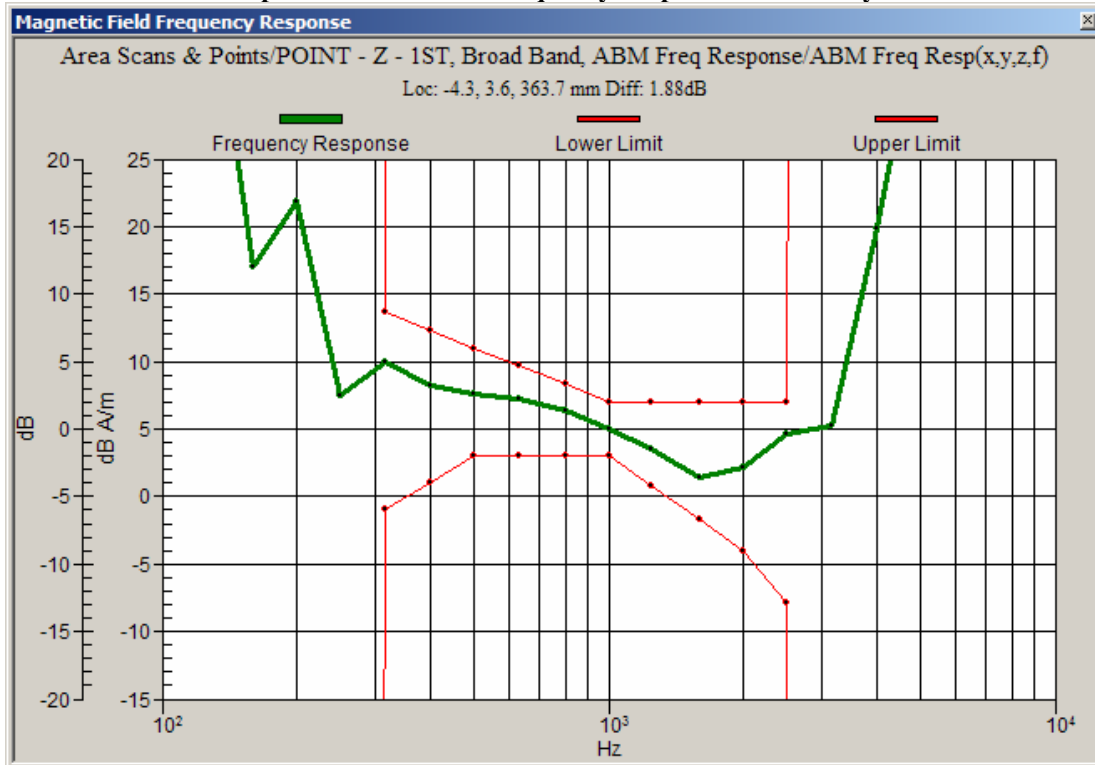
Graph 7: WCDMA 850 Frequency Response with Battery 2
