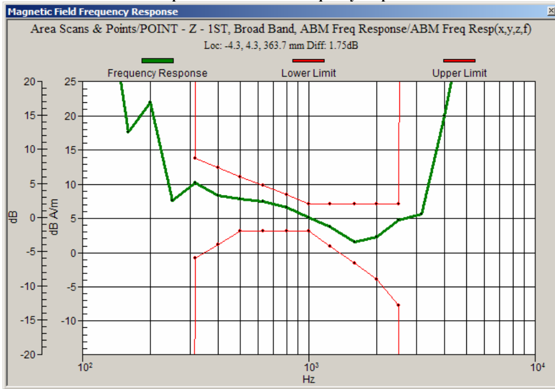
Graph 8: WCDMA 1900 Frequency Response
