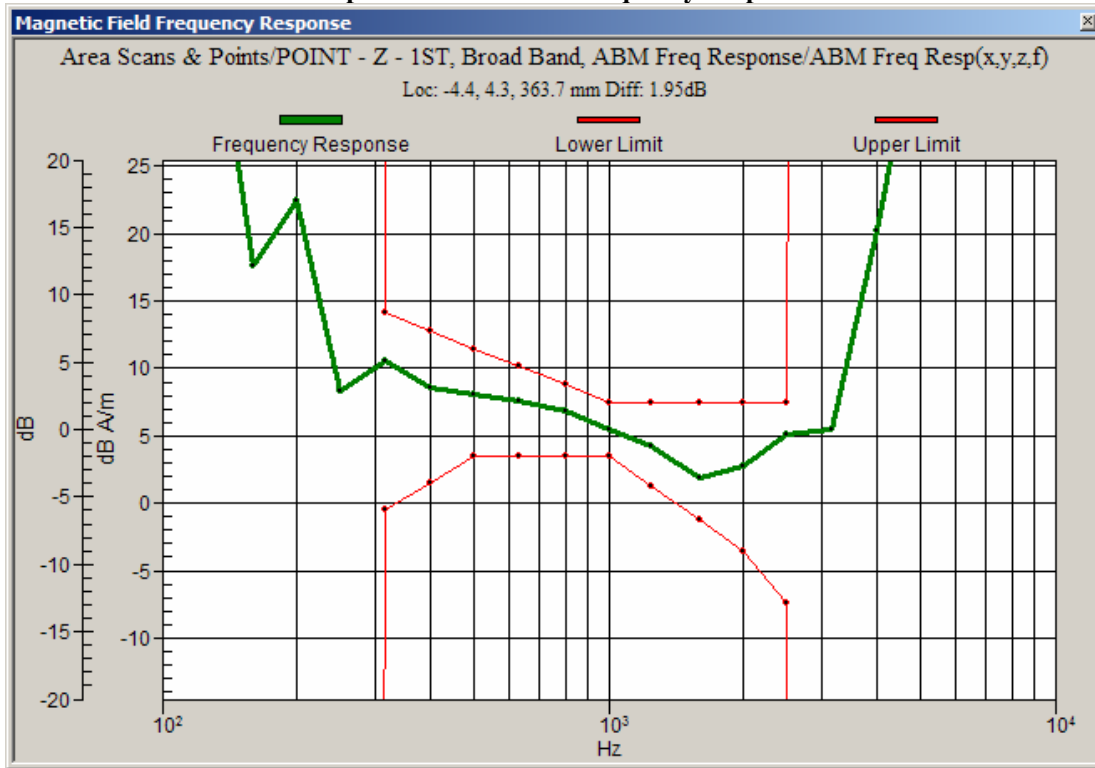
Graph 6: WCDMA 850 Frequency Response
