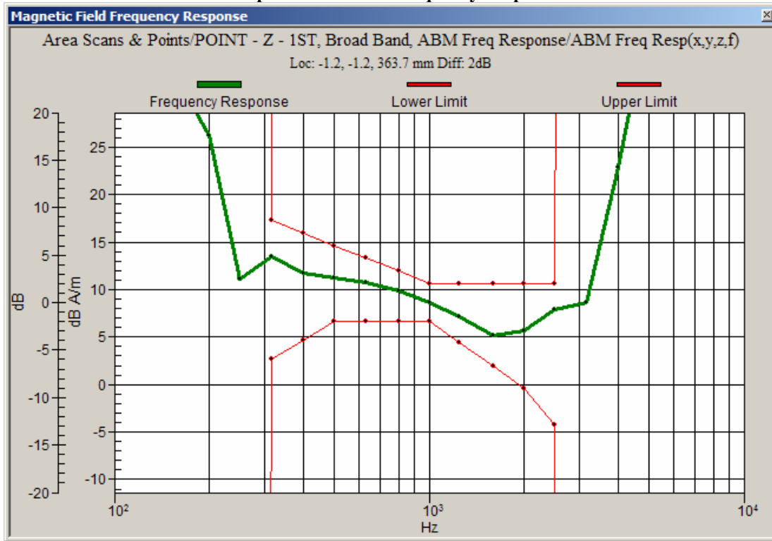
Graph 4: GSM 1900 Frequency Response
