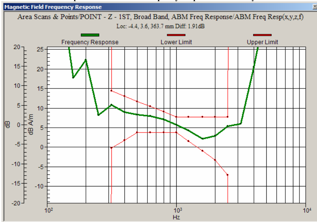
Graph 9: WCDMA 1900 Frequency Response with Battery 2
