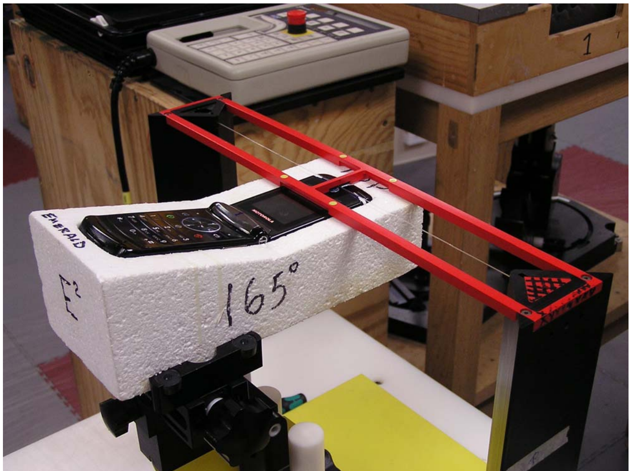
Figure 4. Positioning for RF Emissions
