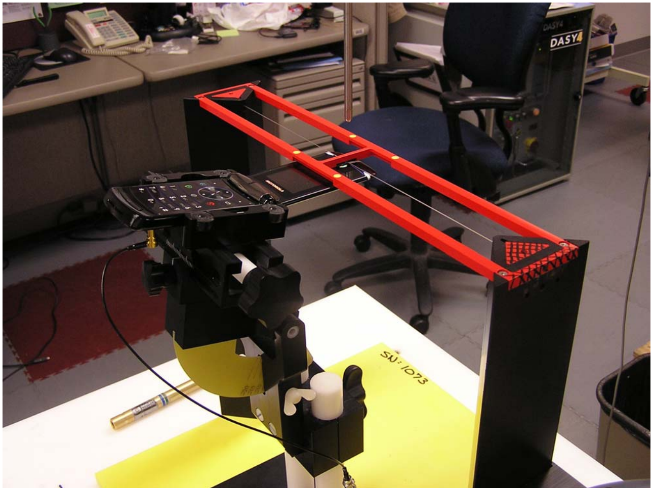
Figure 8. Positioning and Measurement for Telecoil
