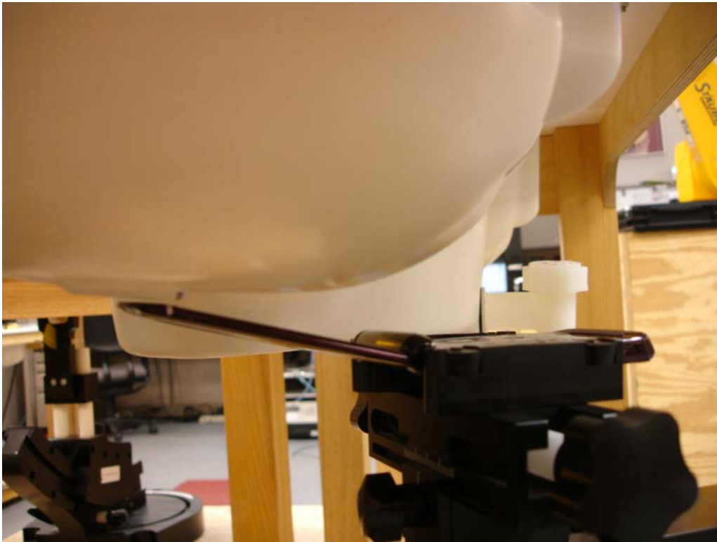
Figure 5. 15° Tilt Position
