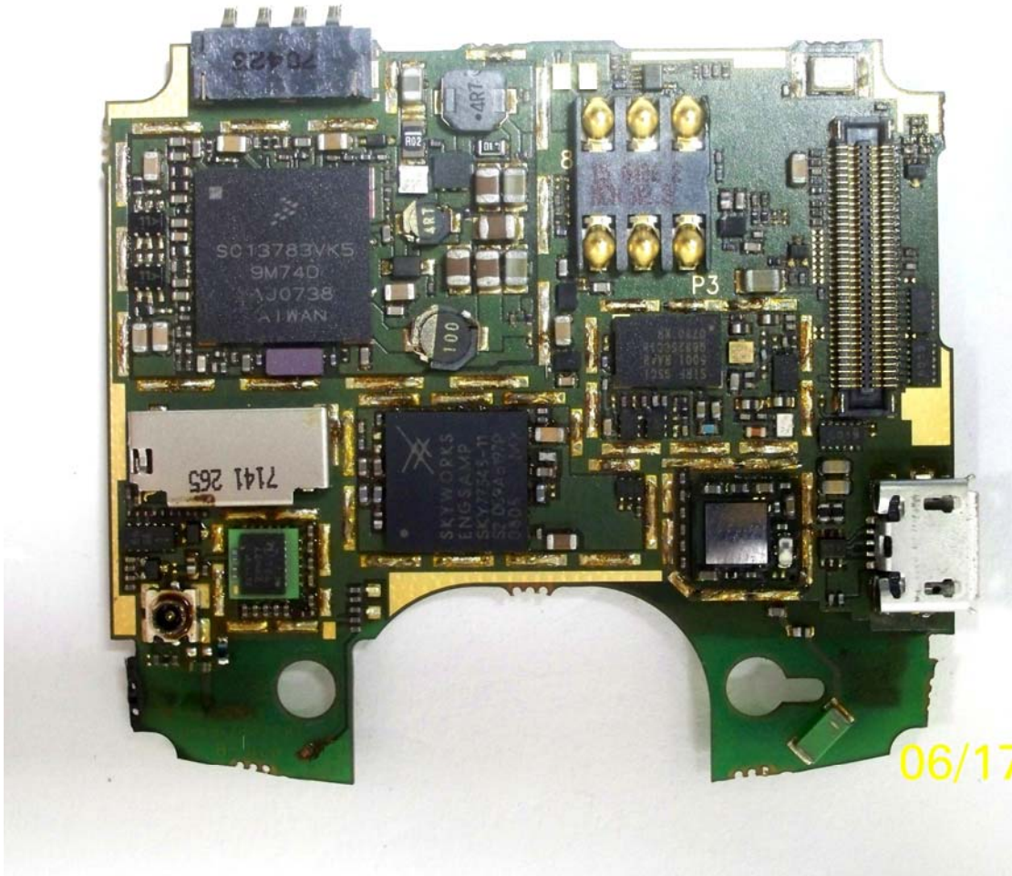
Main Board Bottom Without Shields
