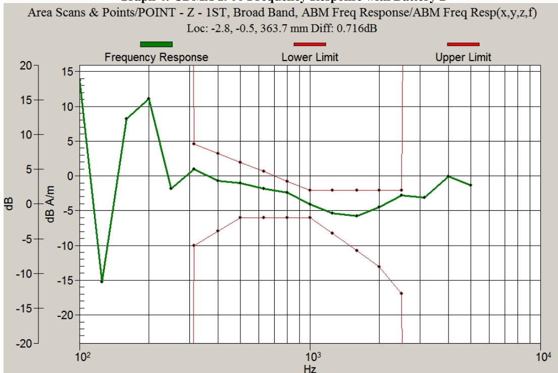
Graph 4: CDMA 1900 Frequency Response with Battery 2
