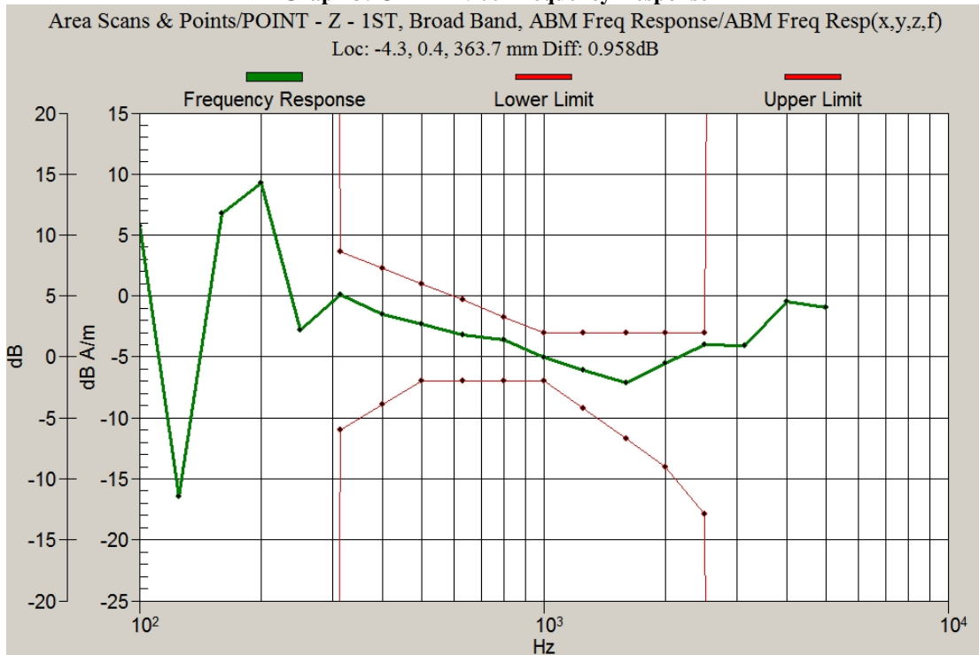
Graph 3: CDMA 1900 Frequency Response
