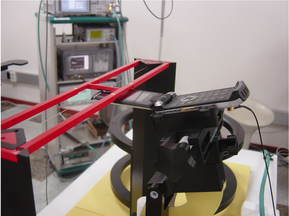
Figure A4-6. Positioning and Measurement for T-coil
