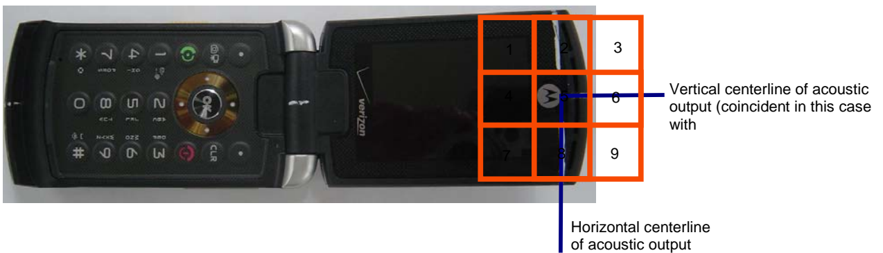
Figure A5-3. Phone Open - Orientation and Measurement Plane for RF Emissions Testing
