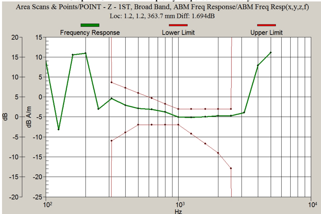
Graph 5: CDMA 1900 Frequency Response with Battery 2
