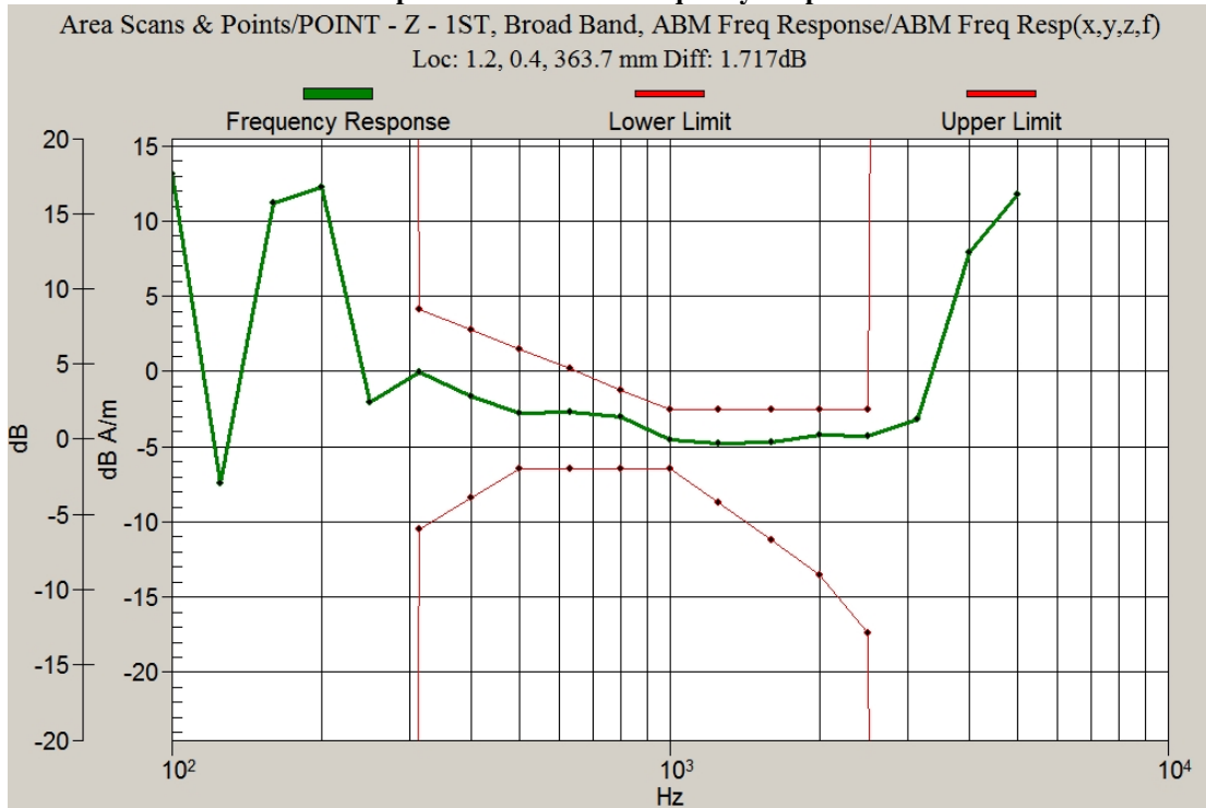
Graph 4: CDMA 1900 Frequency Response
