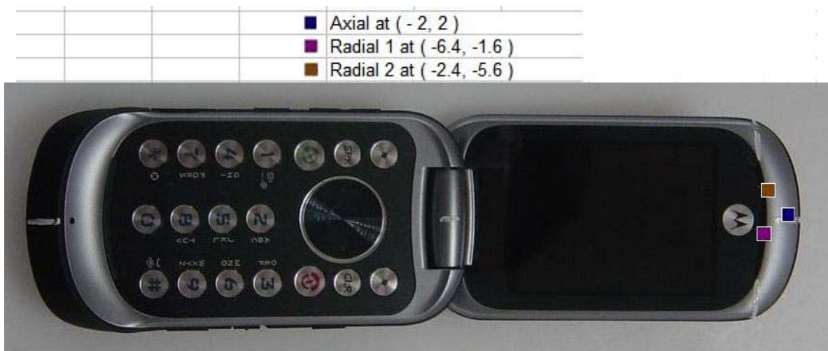
Figure A4-5. Location of Measured Points for T-coil measurements
