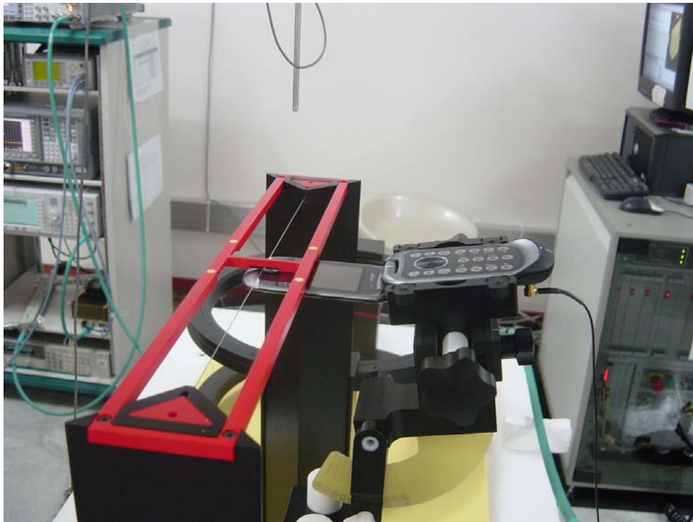
Figure A4-6. Positioning and Measurement for T-coil
