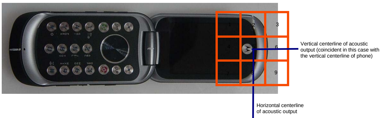
Figure A4-3. Phone Open - Orientation and Measurement Plane for RF Emissions Testing
