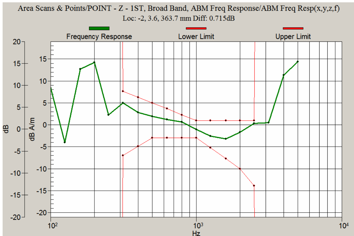
Graph 3: CDMA 800 Frequency Response with Battery 2
