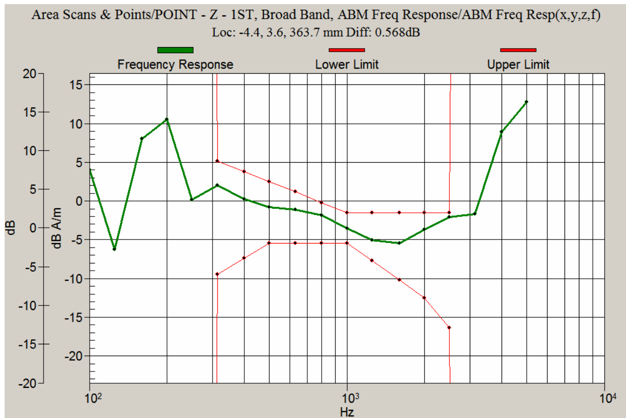
Graph 4: CDMA 1900 Frequency Response with Battery 2
