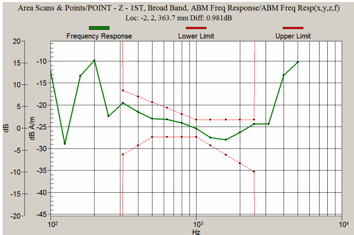
Graph 2: CDMA 800 Frequency Response with Battery 1
