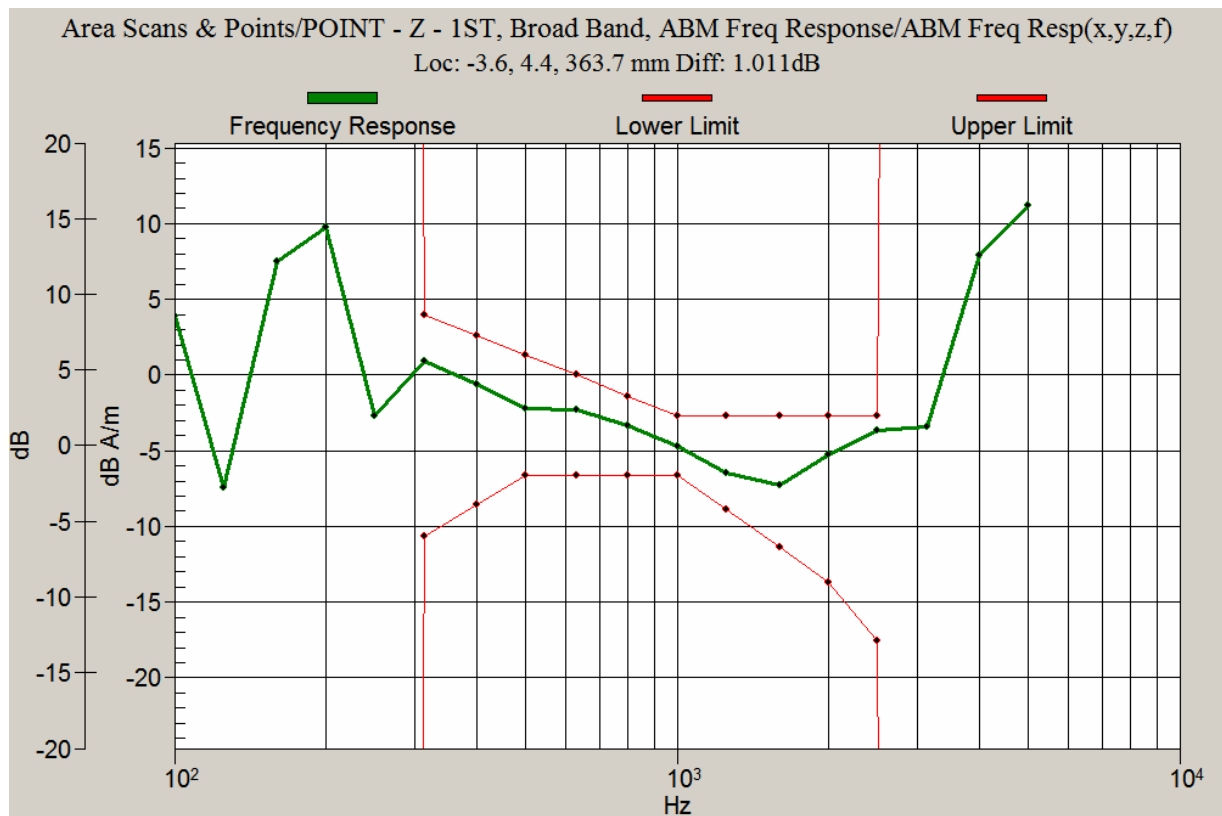
Graph 3: CDMA 1900 Frequency Response with Battery1
