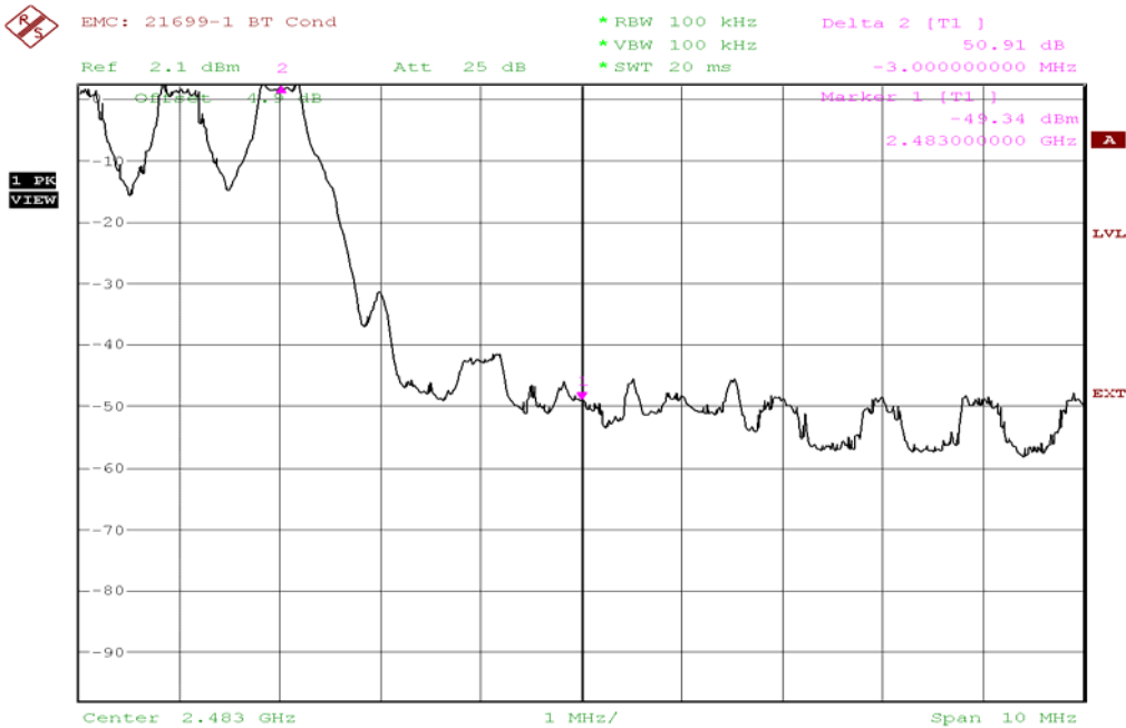
High Band edge with Hopping Disabled
