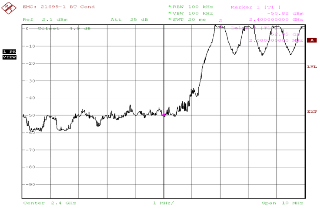
Low Band edge with Hopping Disabled
