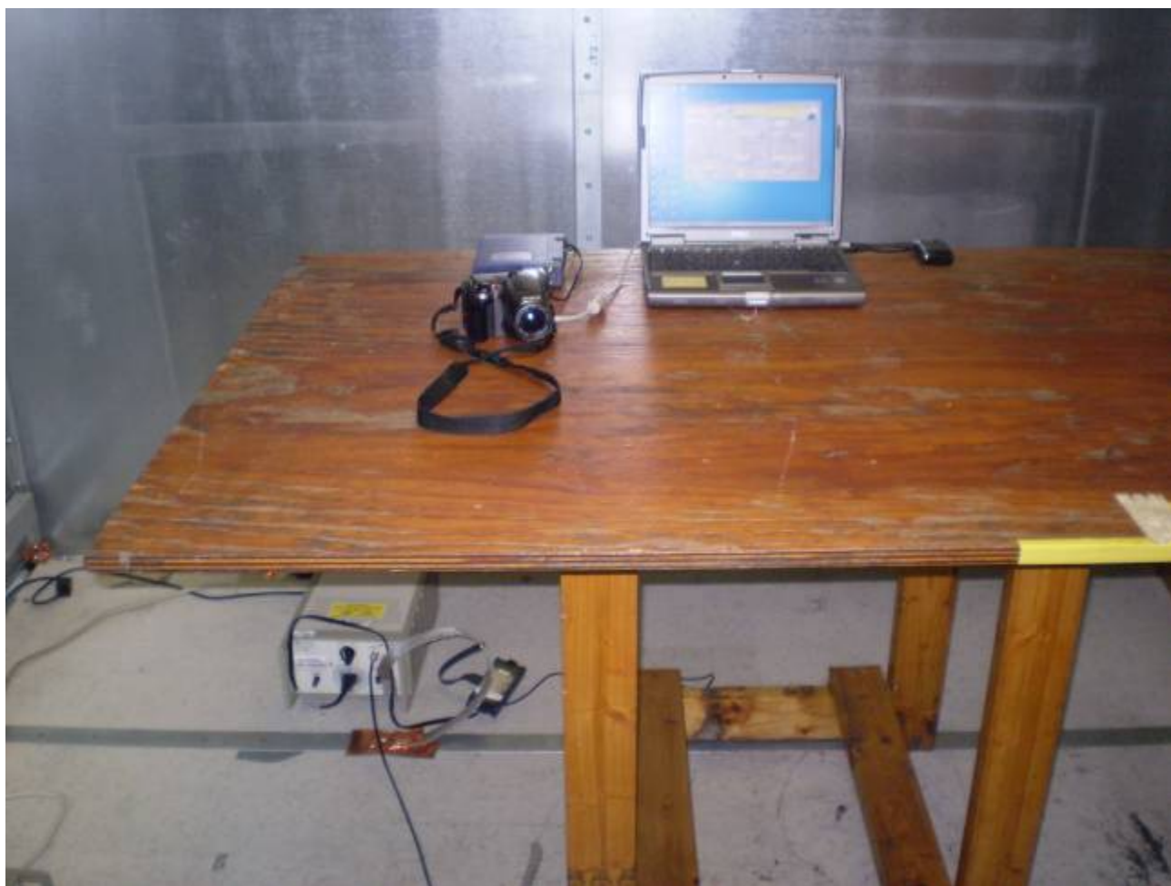
AC Line Conducted Emissions
