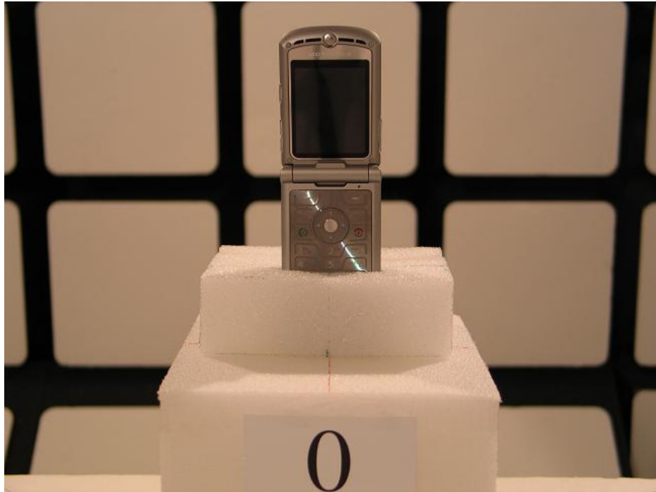
21531-1, IHDT56JE1 placed in test position Z
