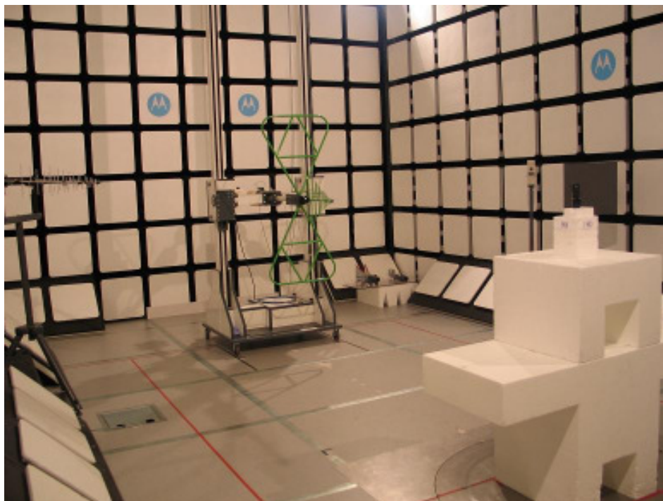
21531-1, IHDT56JE1 setup in semi-anechoic chamber – front view
