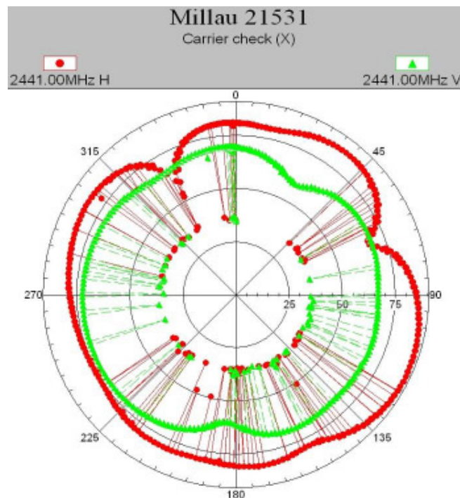
21531-1, IHDT56JE1 maximum radiation pattern position X - Open
