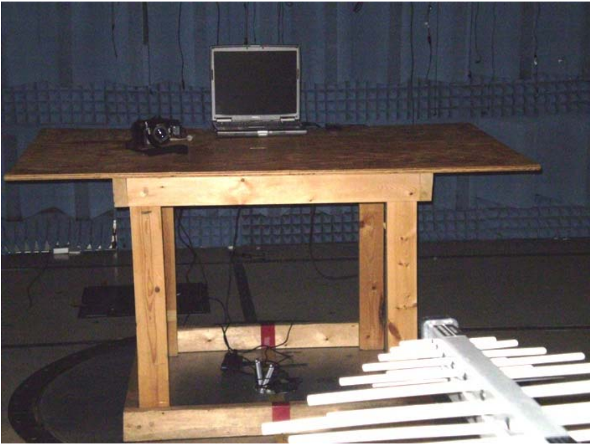
EMC Report #21531 Part 15, PC Peripheral
