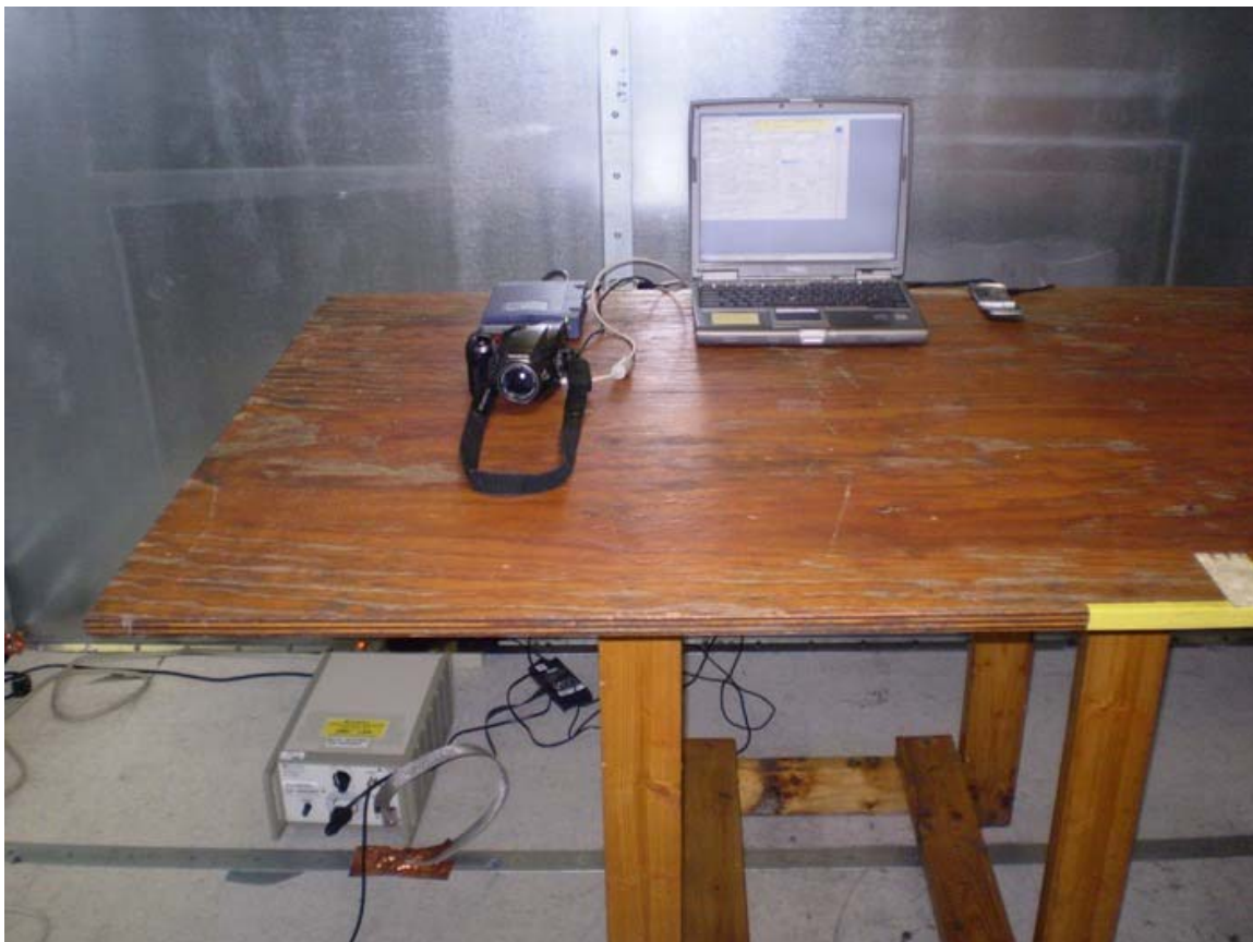
EMC Report #21531 AC Line - Part 15
