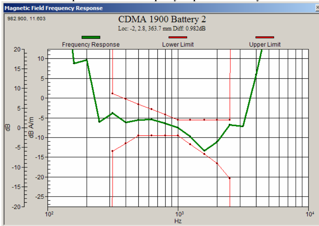
Graph 5: CDMA 1900 Frequency Response with Battery 2
