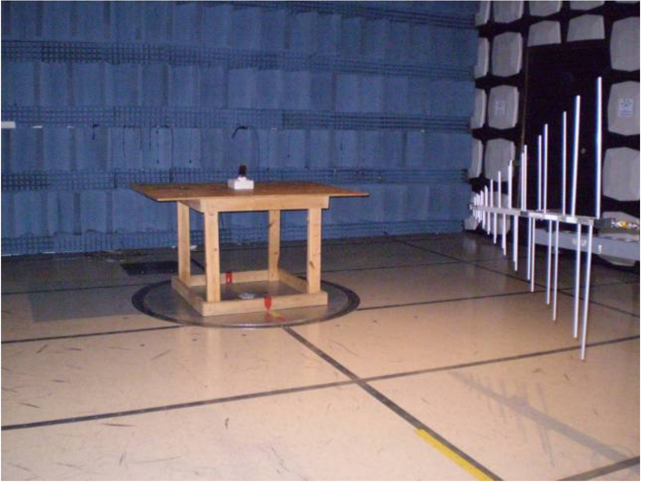
Radiated Emissions
