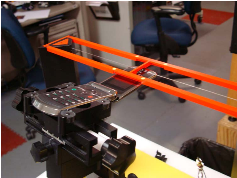
Figure 6. Positioning and Measurement for T-coil
