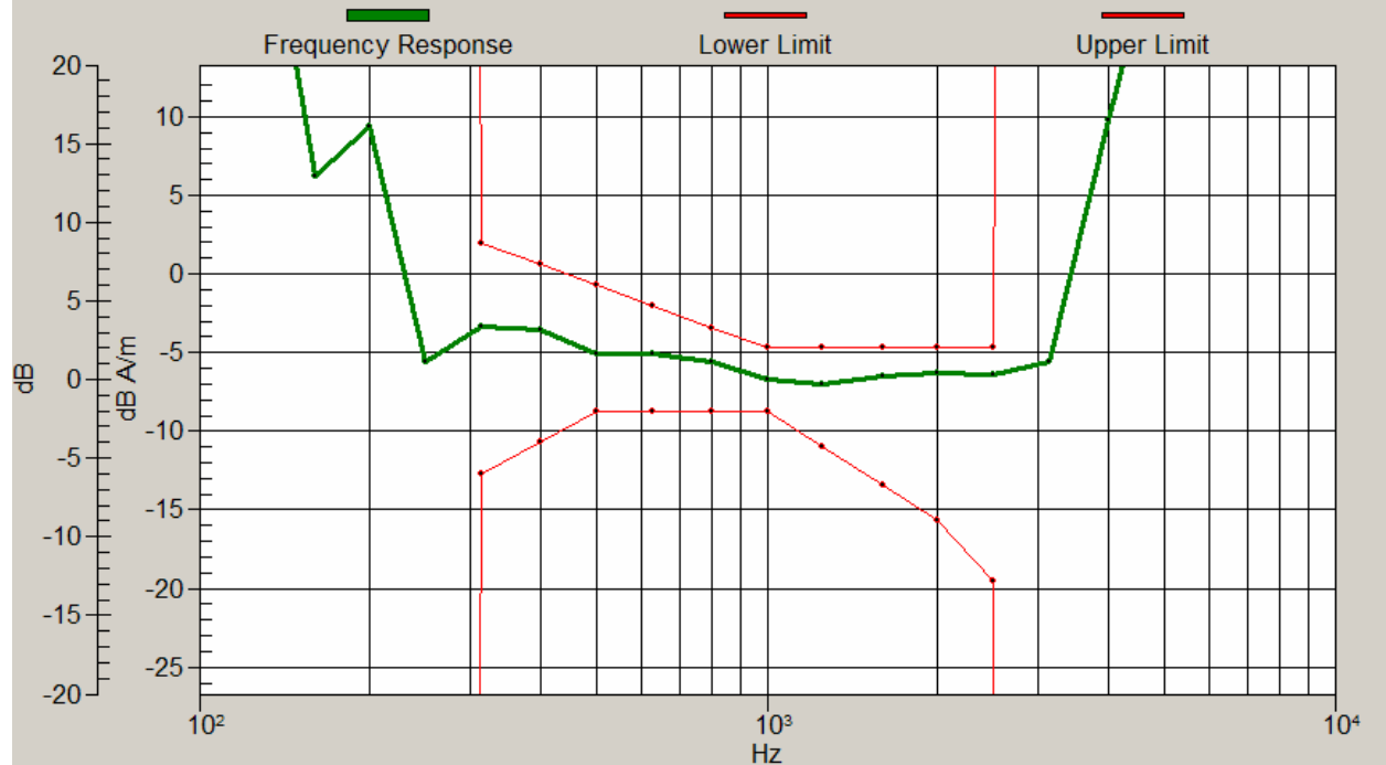
Graph 3: CDMA 800 Frequency Response with Battery 2
