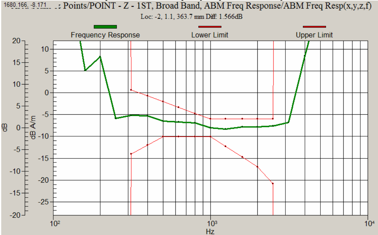
Graph 4: CDMA 800 Frequency Response with Battery 3
