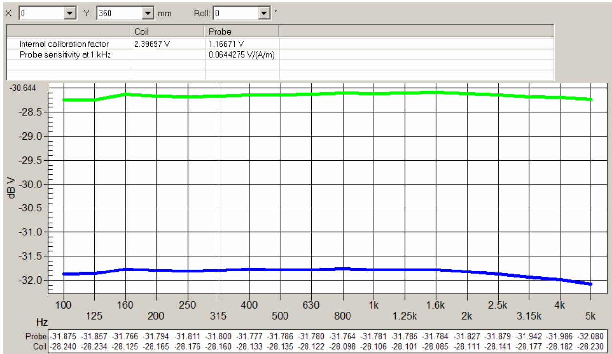
Graph 1: Frequency Response measured in AMCC
