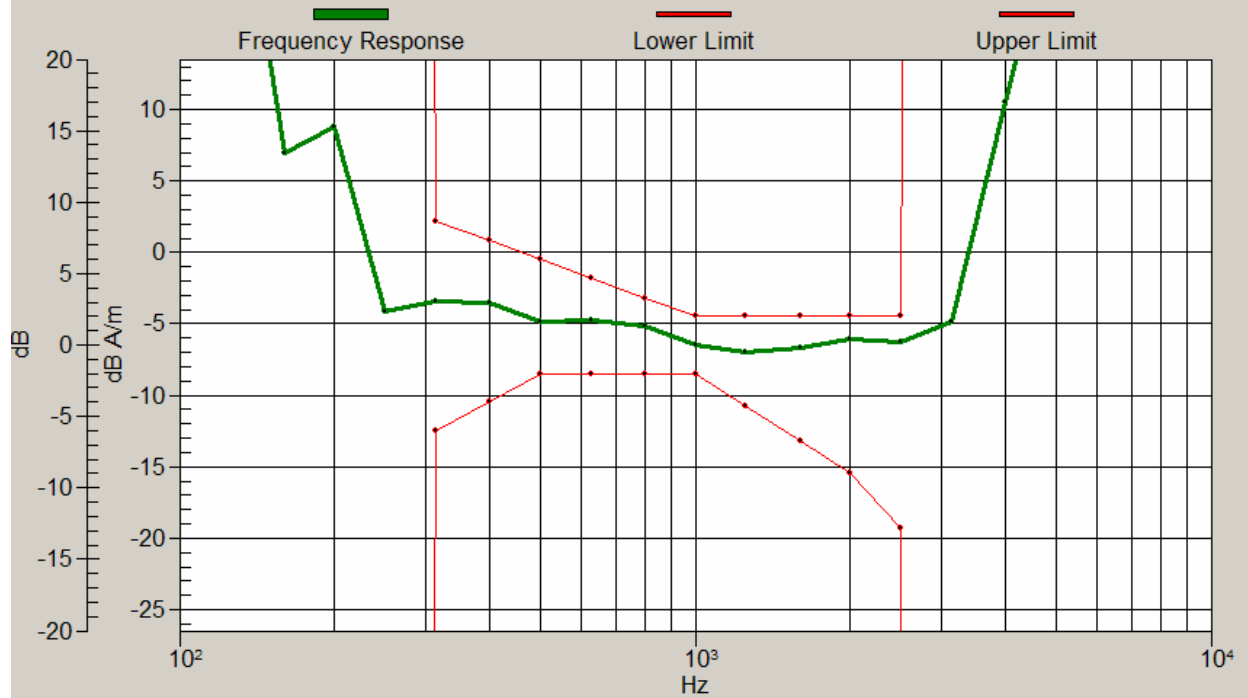
Graph 7: CDMA 1900 Frequency Response with Battery 3
