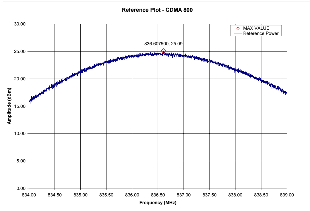
CDMA 800 – Reference Level Plot – Channel 384 (836.52 MHz)
