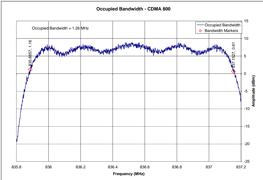
CDMA 800 – Occupied Bandwidth – Channel 384 (836.52MHz)
