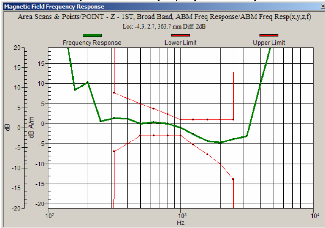
Graph 9: CDMA 1900 Frequency Response with Battery 4
