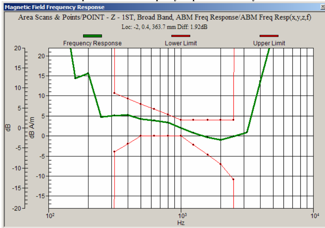
Graph 5: CDMA 800 Frequency Response with Battery 4
