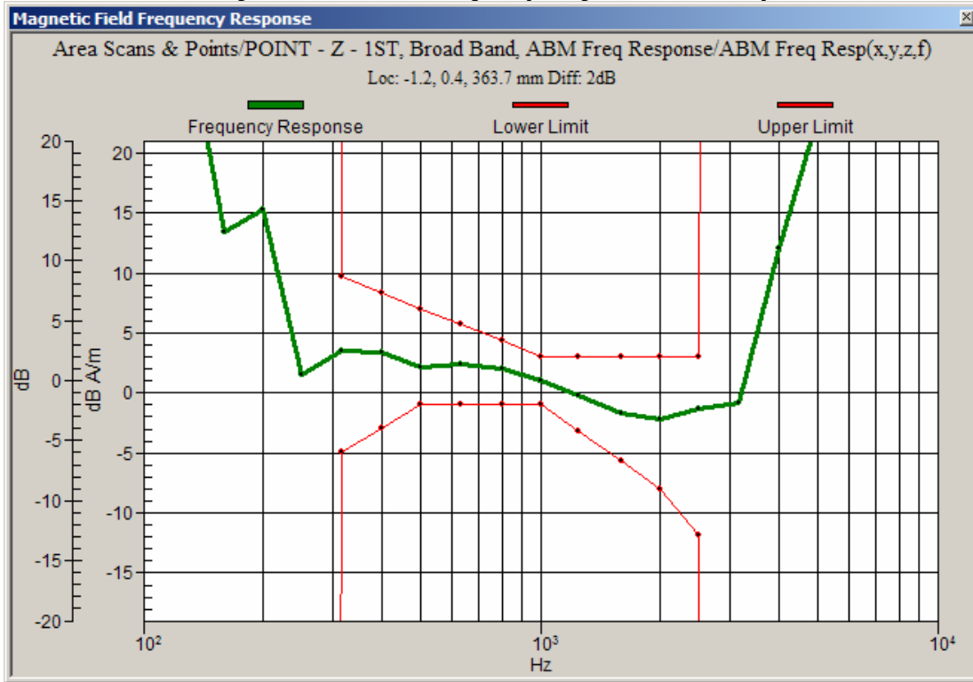
Graph 8: CDMA 1900 Frequency Response with Battery 3
