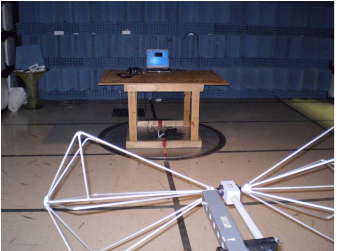
Radiated Emissions
