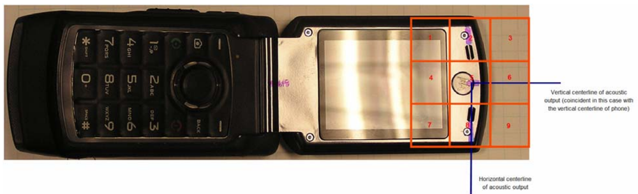
Figure A5-3. Phone Open - Orientation and Measurement Plane for RF Emissions Testing
