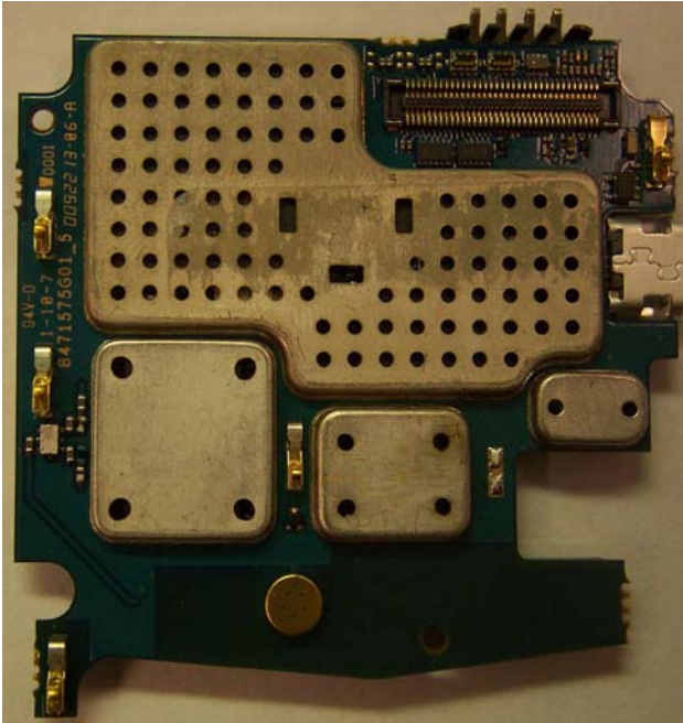
Main Board Top With Shields
