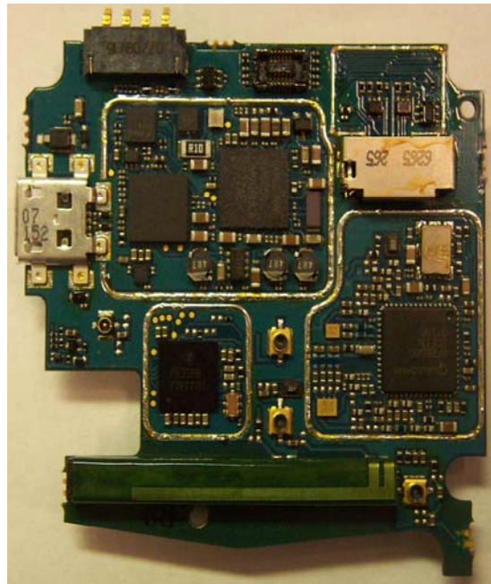
Main Board Bottom Without Shields
