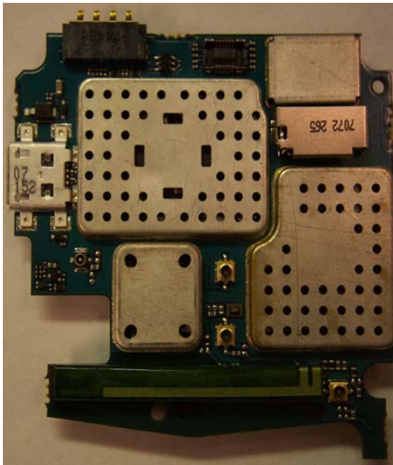
Main Board Bottom With Shields
