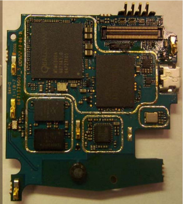
Main Board Top Without Shields
