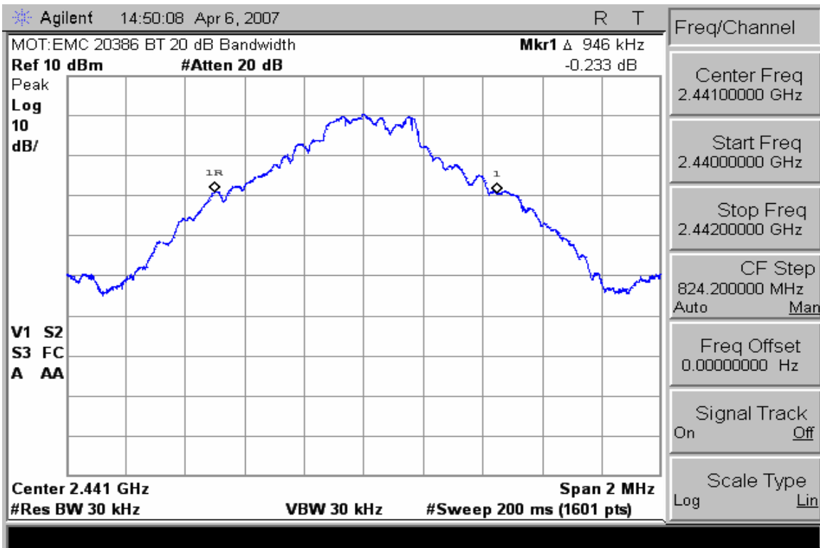
20 dB Bandwidth
