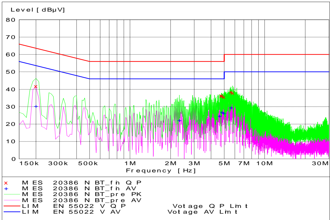
Bluetooth - Hopping Mode - Neutral Coupling
