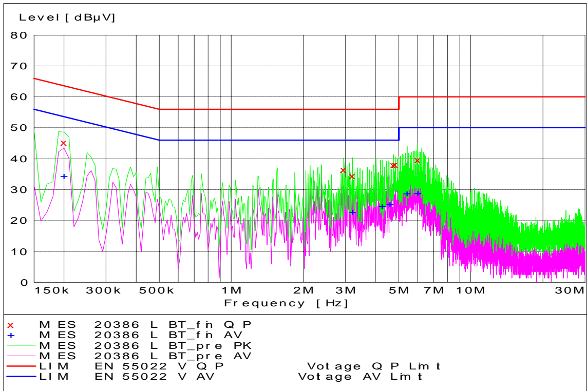
Bluetooth - Hopping Mode – Line Coupling
