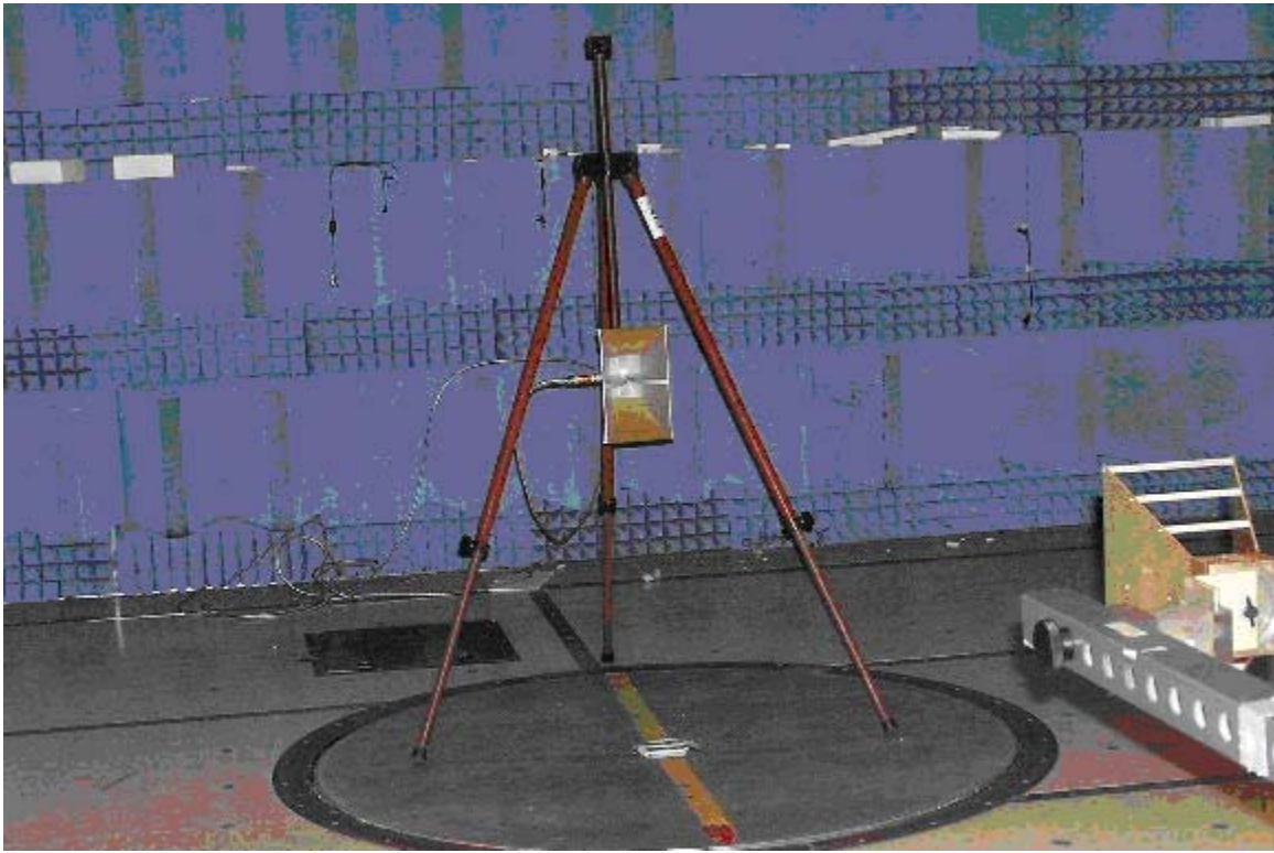
Motorola EMC Report #19881-1, Antenna - Substitution
