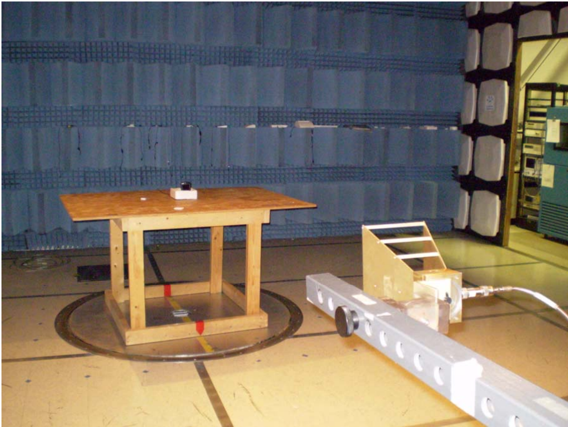
Motorola EMC Report #19881-1, Tx Radiated
