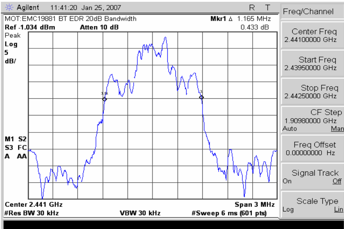
20dB Bandwidth EDR Enabled
