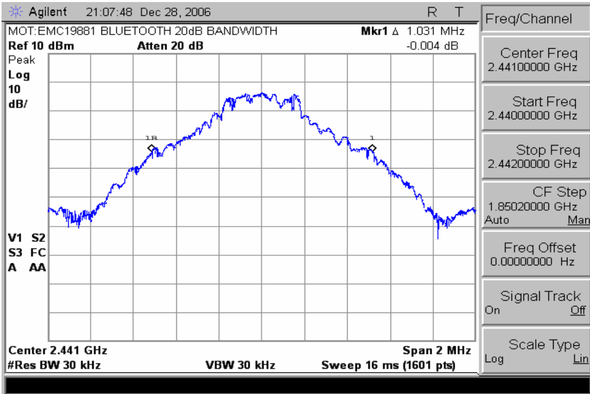
20dB Bandwidth EDR Disabled
